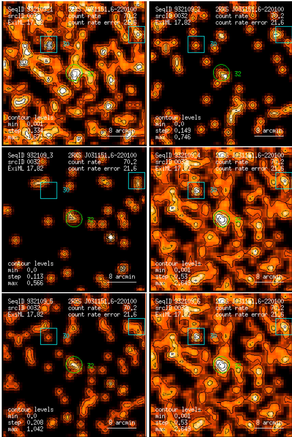
Figure 32: RASS 932109: detection 0032: band rate images, Gaussian filter: (1) PSPC channels 11 – 41, (2) 52 – 90, (3) 91 – 201, (4) 11 – 235, (5) 52 – 201, (6) 11 – 201. Broad band rates in counts/ks. Band rate contour levels in counts/ks/arcmin 2 .
