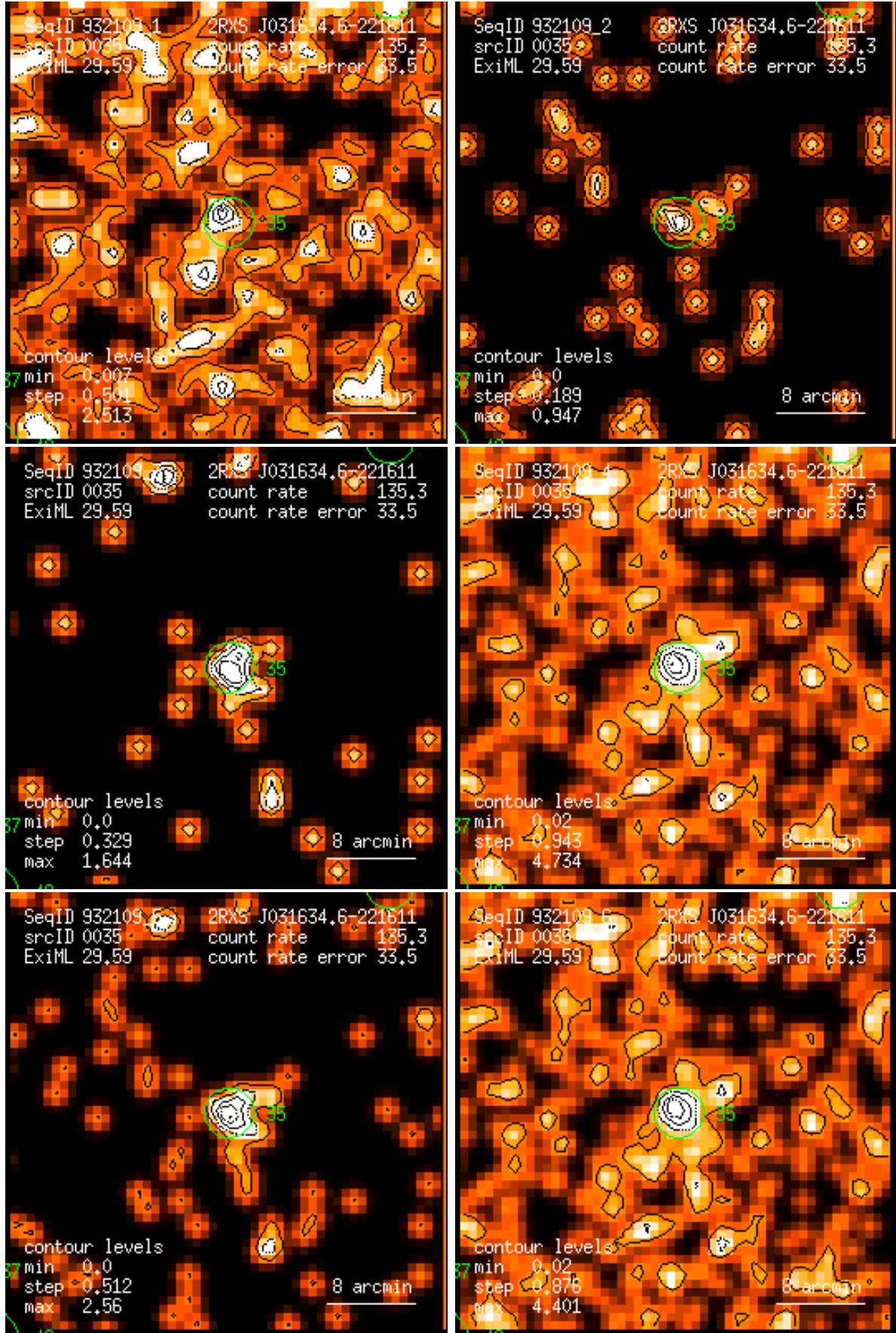
Figure 35: RASS 932109: detection 0035: band rate images, Gaussian filter: (1) PSPC channels 11 – 41, (2) 52 – 90, (3) 91 – 201, (4) 11 – 235, (5) 52 – 201, (6) 11 – 201. Broad band rates in counts/ks. Band rate contour levels in counts/ks/arcmin 2 .
