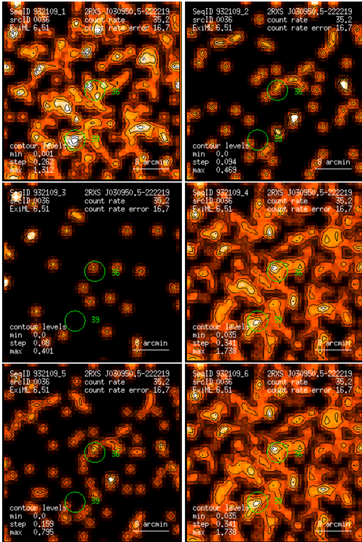
Figure 36: RASS 932109: detection 0036: band rate images, Gaussian filter: (1) PSPC channels 11 – 41, (2) 52 – 90, (3) 91 – 201, (4) 11 – 235, (5) 52 – 201, (6) 11 – 201. Broad band rates in counts/ks. Band rate contour levels in counts/ks/arcmin 2 .
