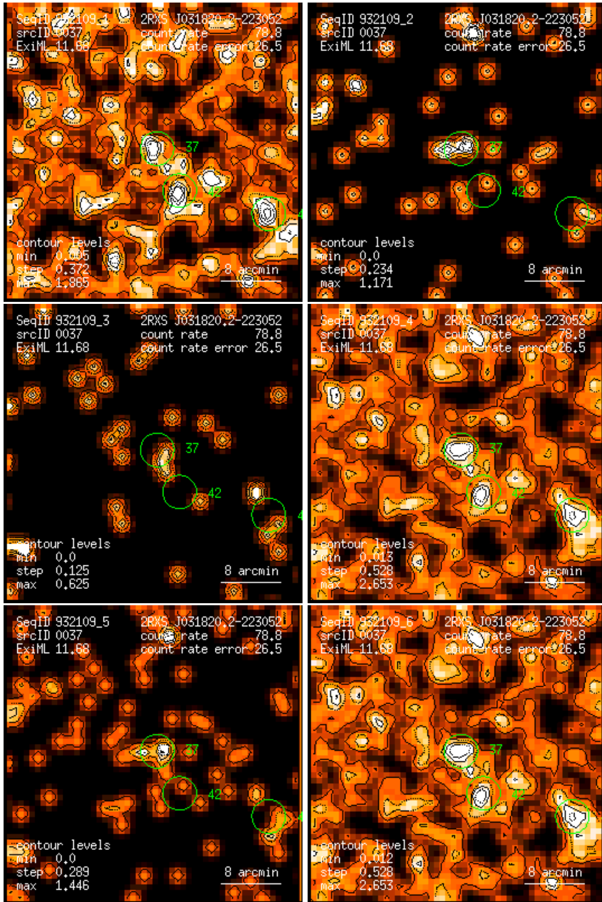
Figure 37: RASS 932109: detection 0037: band rate images, Gaussian filter: (1) PSPC channels 11 – 41, (2) 52 – 90, (3) 91 – 201, (4) 11 – 235, (5) 52 – 201, (6) 11 – 201. Broad band rates in counts/ks. Band rate contour levels in counts/ks/arcmin 2 .
