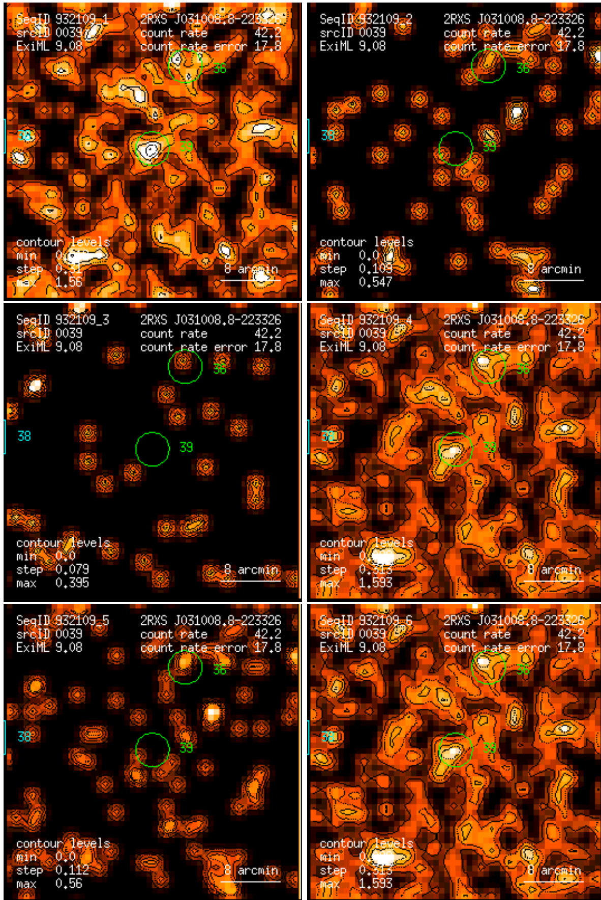
Figure 39: RASS 932109: detection 0039: band rate images, Gaussian filter: (1) PSPC channels 11 – 41, (2) 52 – 90, (3) 91 – 201, (4) 11 – 235, (5) 52 – 201, (6) 11 – 201. Broad band rates in counts/ks. Band rate contour levels in counts/ks/arcmin 2 .
