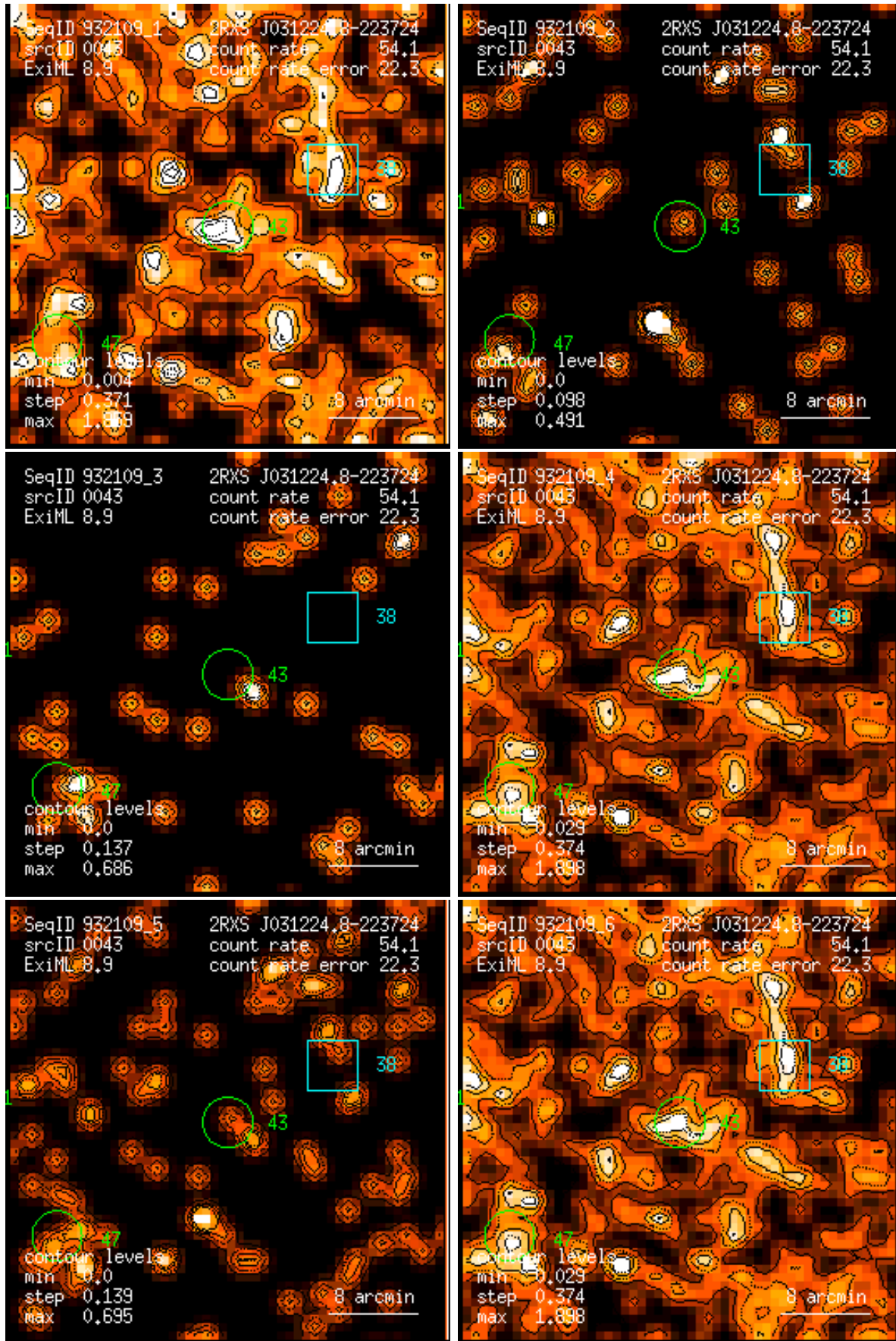
Figure 43: RASS 932109: detection 0043: band rate images, Gaussian filter: (1) PSPC channels 11 – 41, (2) 52 – 90, (3) 91 – 201, (4) 11 – 235, (5) 52 – 201, (6) 11 – 201. Broad band rates in counts/ks. Band rate contour levels in counts/ks/arcmin 2 .
