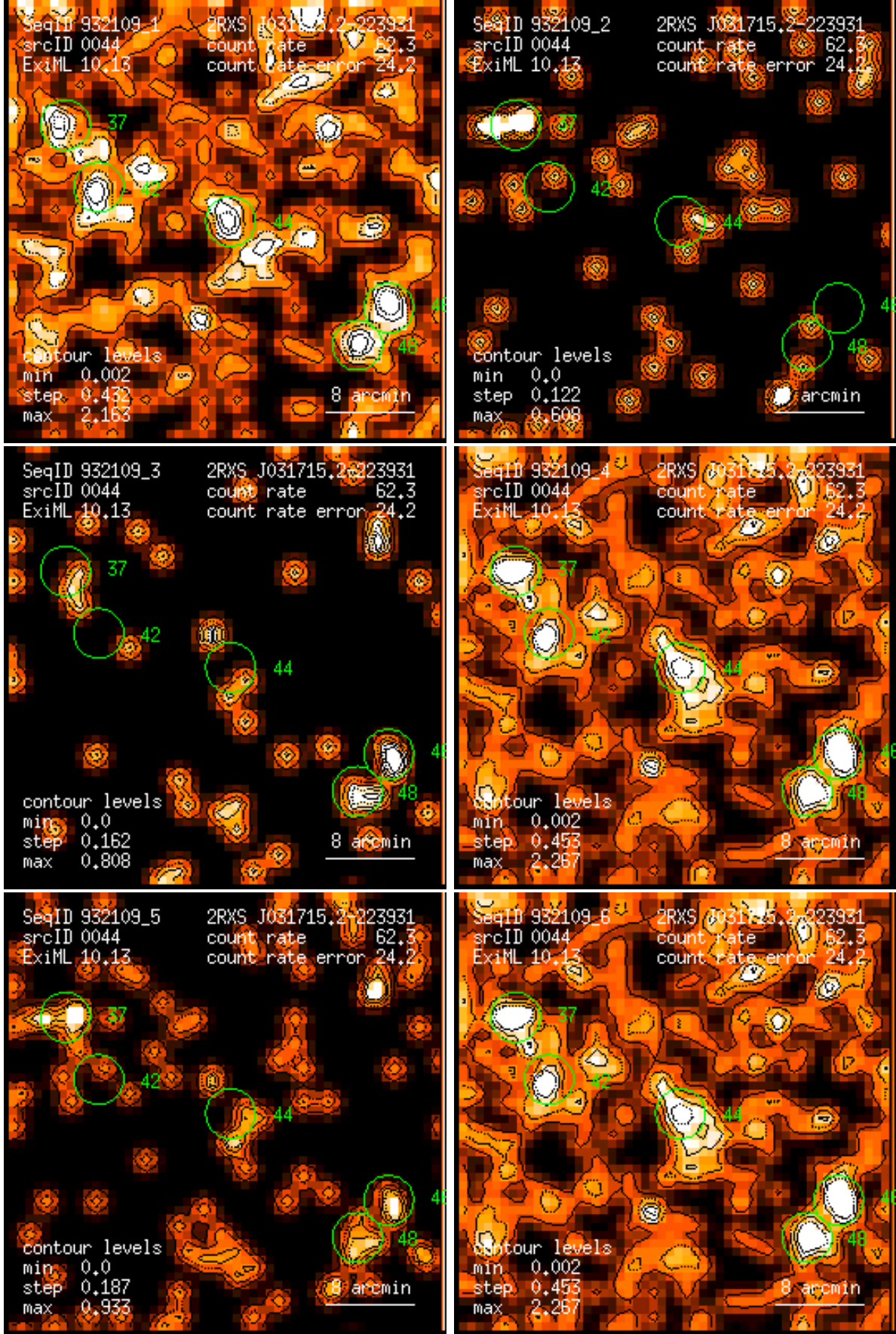
Figure 44: RASS 932109: detection 0044: band rate images, Gaussian filter: (1) PSPC channels 11 – 41, (2) 52 – 90, (3) 91 – 201, (4) 11 – 235, (5) 52 – 201, (6) 11 – 201. Broad band rates in counts/ks. Band rate contour levels in counts/ks/arcmin 2 .
