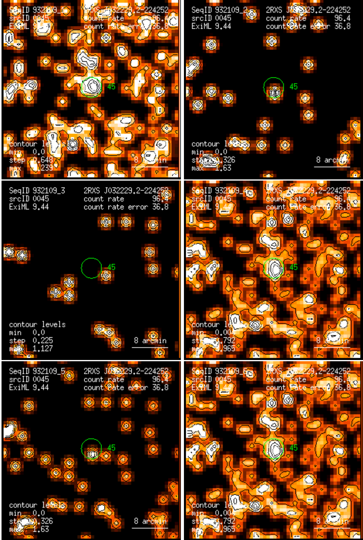
Figure 45: RASS 932109: detection 0045: band rate images, Gaussian filter: (1) PSPC channels 11 – 41, (2) 52 – 90, (3) 91 – 201, (4) 11 – 235, (5) 52 – 201, (6) 11 – 201. Broad band rates in counts/ks. Band rate contour levels in counts/ks/arcmin 2 .
