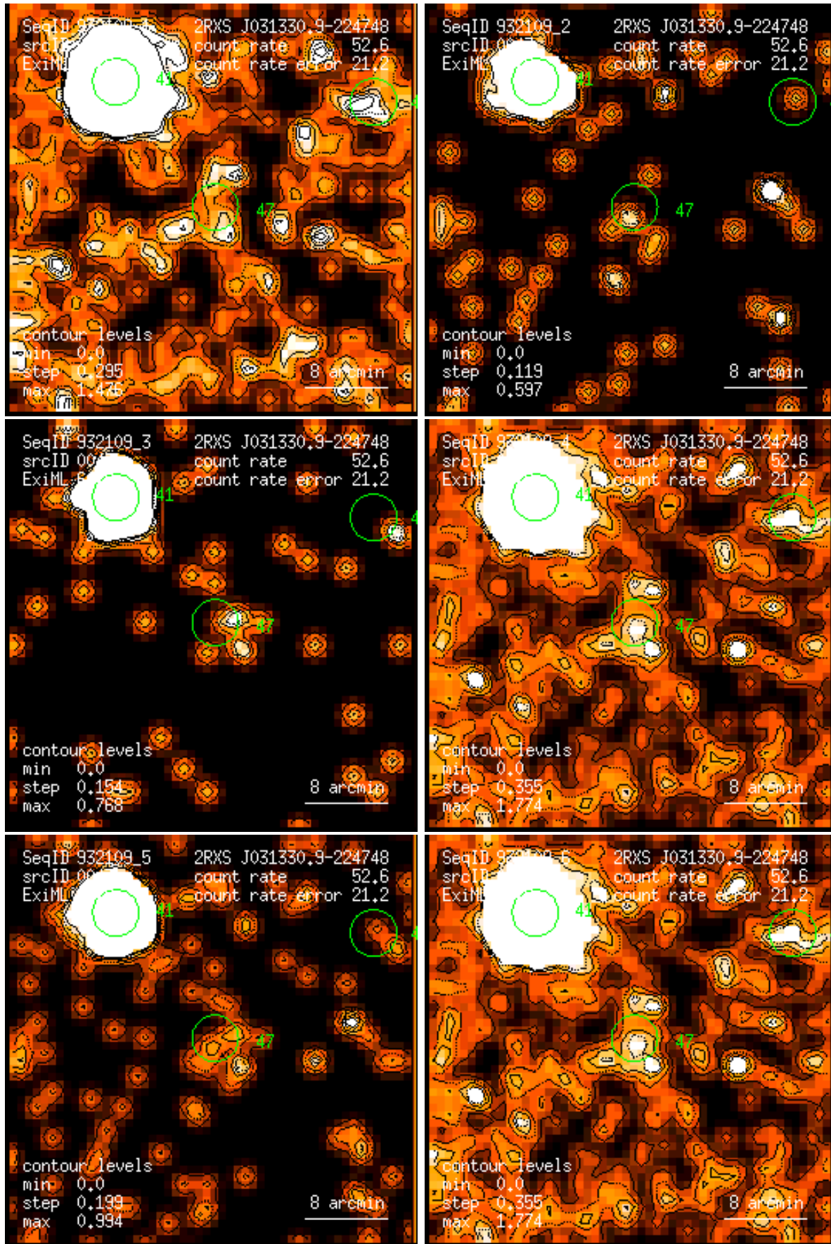
Figure 47: RASS 932109: detection 0047: band rate images, Gaussian filter: (1) PSPC channels 11 – 41, (2) 52 – 90, (3) 91 – 201, (4) 11 – 235, (5) 52 – 201, (6) 11 – 201. Broad band rates in counts/ks. Band rate contour levels in counts/ks/arcmin 2 .
