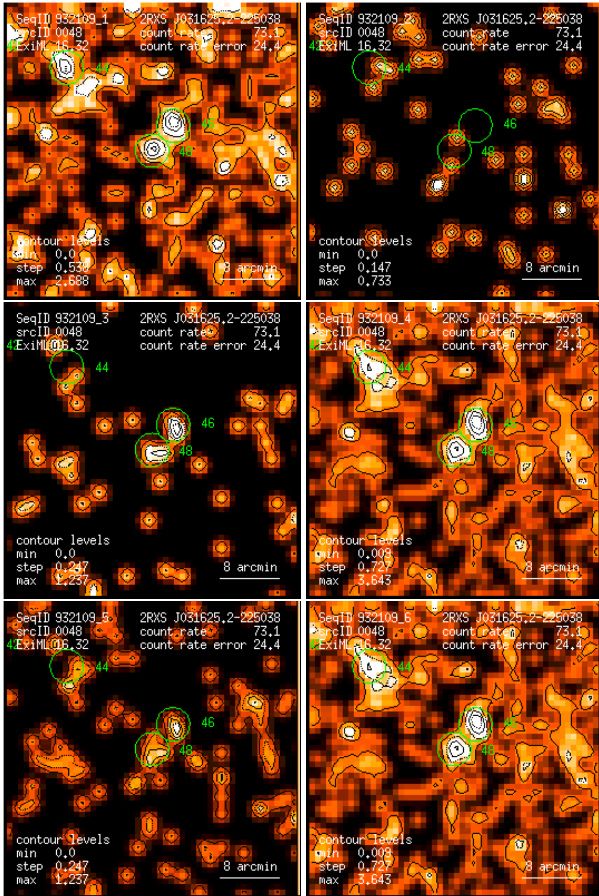
Figure 48: RASS 932109: detection 0048: band rate images, Gaussian filter: (1) PSPC channels 11 – 41, (2) 52 – 90, (3) 91 – 201, (4) 11 – 235, (5) 52 – 201, (6) 11 – 201. Broad band rates in counts/ks. Band rate contour levels in counts/ks/arcmin 2 .
