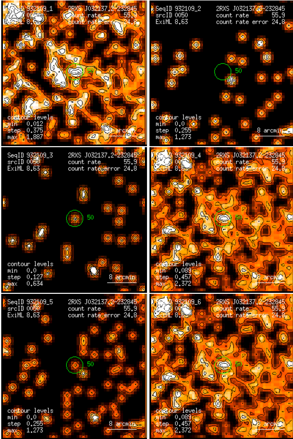
Figure 50: RASS 932109: detection 0050: band rate images, Gaussian filter: (1) PSPC channels 11 – 41, (2) 52 – 90, (3) 91 – 201, (4) 11 – 235, (5) 52 – 201, (6) 11 – 201. Broad band rates in counts/ks. Band rate contour levels in counts/ks/arcmin 2 .
