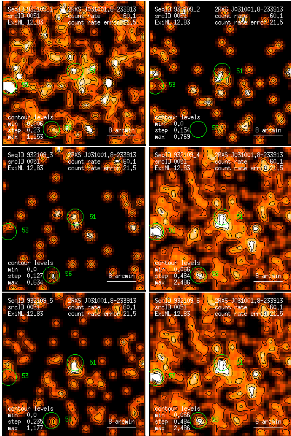
Figure 51: RASS 932109: detection 0051: band rate images, Gaussian filter: (1) PSPC channels 11 – 41, (2) 52 – 90, (3) 91 – 201, (4) 11 – 235, (5) 52 – 201, (6) 11 – 201. Broad band rates in counts/ks. Band rate contour levels in counts/ks/arcmin 2 .
