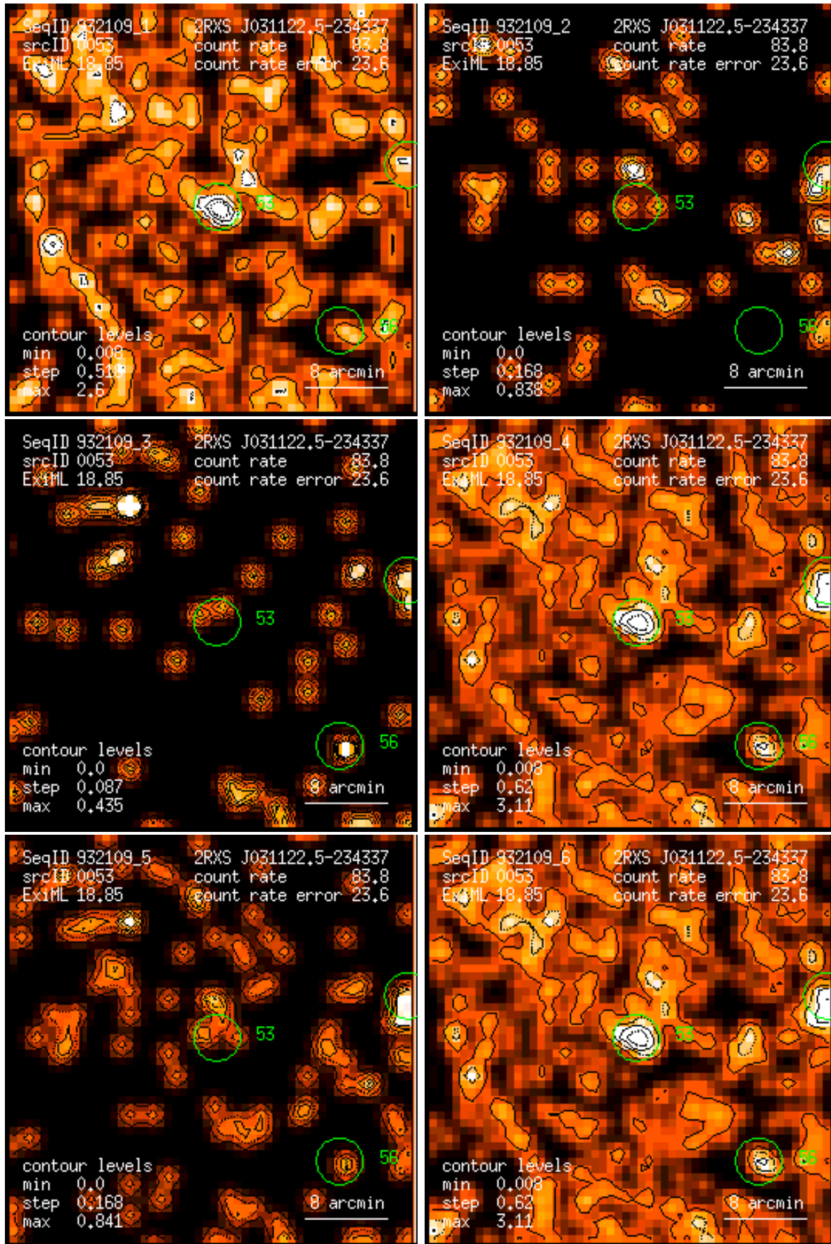
Figure 53: RASS 932109: detection 0053: band rate images, Gaussian filter: (1) PSPC channels 11 – 41, (2) 52 – 90, (3) 91 – 201, (4) 11 – 235, (5) 52 – 201, (6) 11 – 201. Broad band rates in counts/ks. Band rate contour levels in counts/ks/arcmin 2 .
