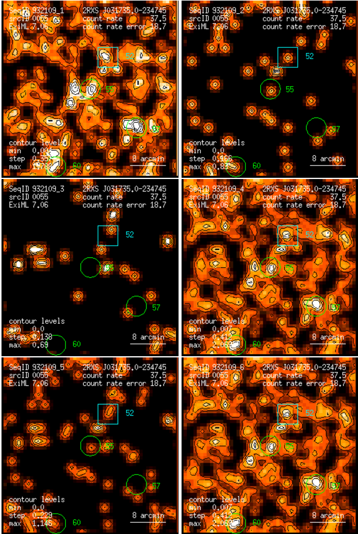
Figure 55: RASS 932109: detection 0055: band rate images, Gaussian filter: (1) PSPC channels 11 – 41, (2) 52 – 90, (3) 91 – 201, (4) 11 – 235, (5) 52 – 201, (6) 11 – 201. Broad band rates in counts/ks. Band rate contour levels in counts/ks/arcmin 2 .
