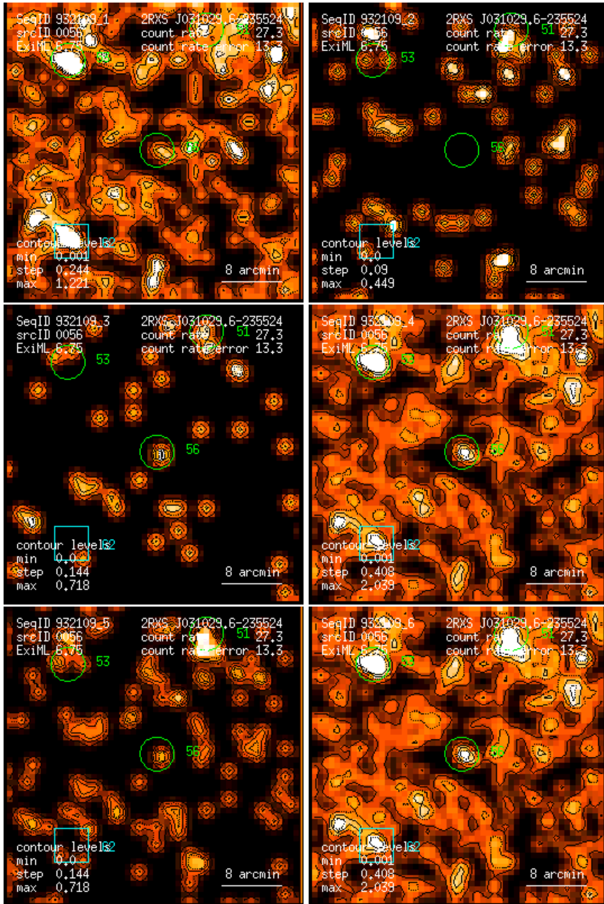
Figure 56: RASS 932109: detection 0056: band rate images, Gaussian filter: (1) PSPC channels 11 – 41, (2) 52 – 90, (3) 91 – 201, (4) 11 – 235, (5) 52 – 201, (6) 11 – 201. Broad band rates in counts/ks. Band rate contour levels in counts/ks/arcmin 2 .
