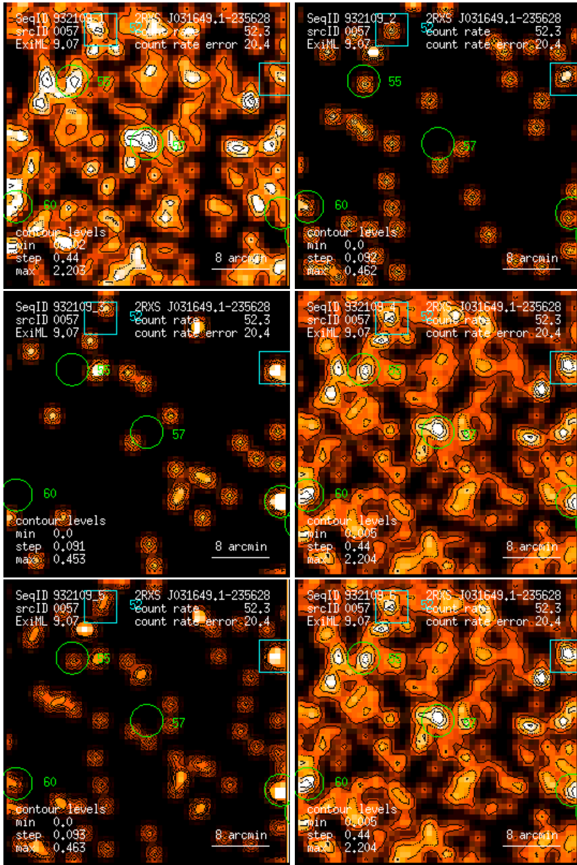
Figure 57: RASS 932109: detection 0057: band rate images, Gaussian filter: (1) PSPC channels 11 – 41, (2) 52 – 90, (3) 91 – 201, (4) 11 – 235, (5) 52 – 201, (6) 11 – 201. Broad band rates in counts/ks. Band rate contour levels in counts/ks/arcmin 2 .
