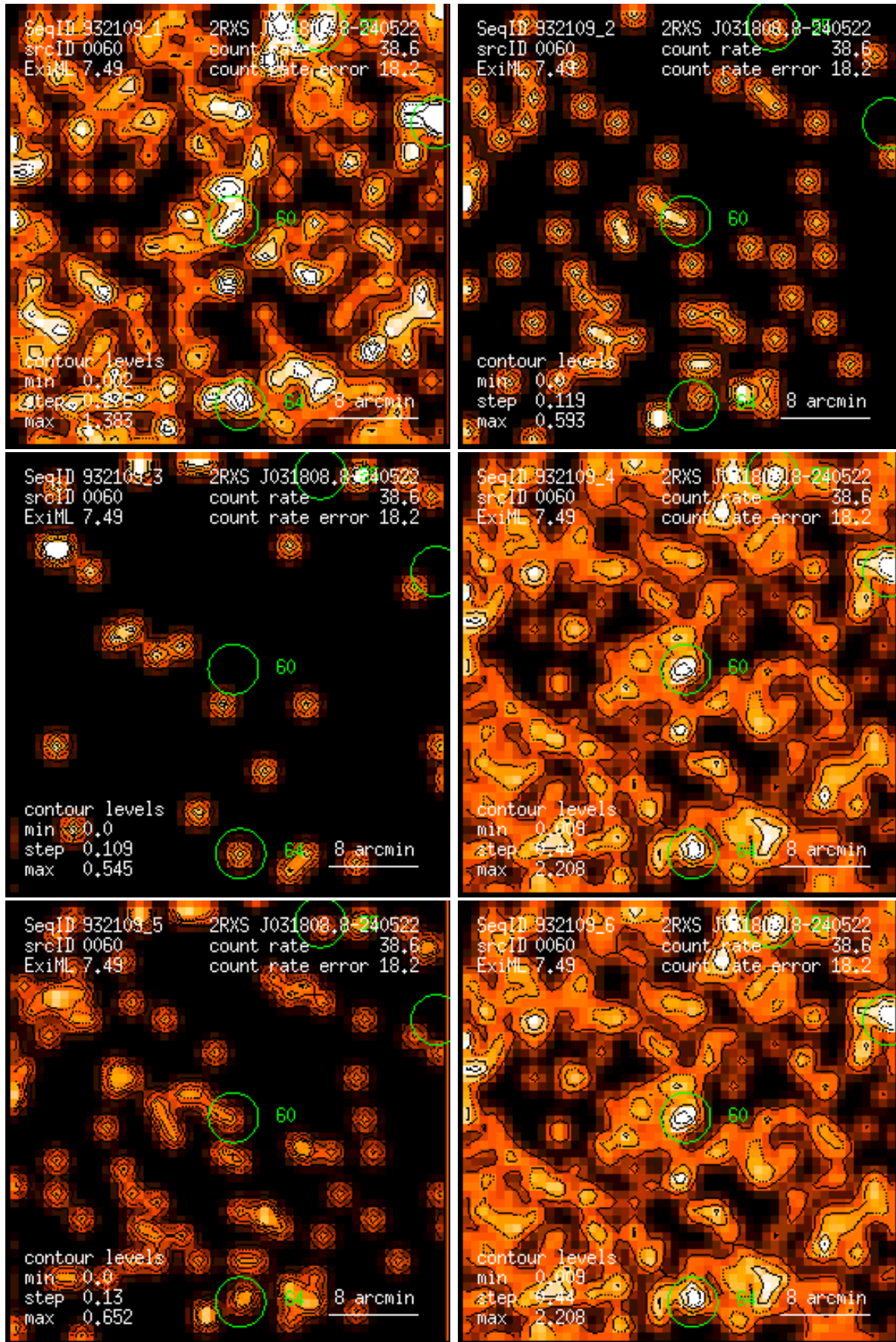
Figure 60: RASS 932109: detection 0060: band rate images, Gaussian filter: (1) PSPC channels 11 – 41, (2) 52 – 90, (3) 91 – 201, (4) 11 – 235, (5) 52 – 201, (6) 11 – 201. Broad band rates in counts/ks. Band rate contour levels in counts/ks/arcmin 2 .
