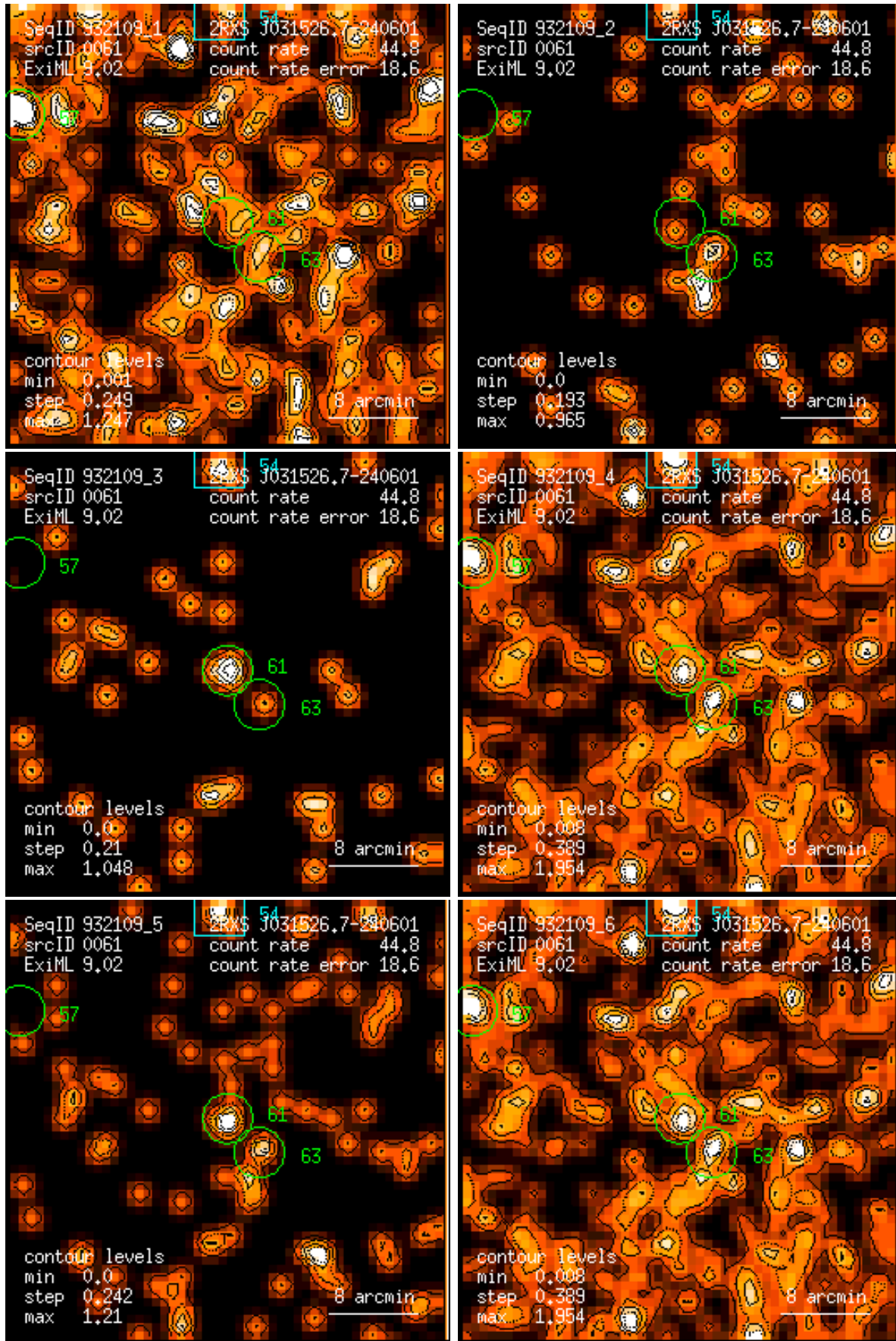
Figure 61: RASS 932109: detection 0061: band rate images, Gaussian filter: (1) PSPC channels 11 – 41, (2) 52 – 90, (3) 91 – 201, (4) 11 – 235, (5) 52 – 201, (6) 11 – 201. Broad band rates in counts/ks. Band rate contour levels in counts/ks/arcmin 2 .
