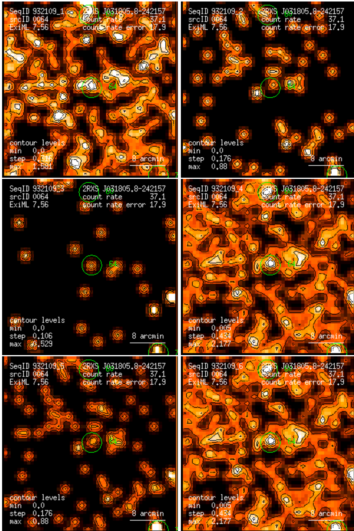
Figure 64: RASS 932109: detection 0064: band rate images, Gaussian filter: (1) PSPC channels 11 – 41, (2) 52 – 90, (3) 91 – 201, (4) 11 – 235, (5) 52 – 201, (6) 11 – 201. Broad band rates in counts/ks. Band rate contour levels in counts/ks/arcmin 2 .
