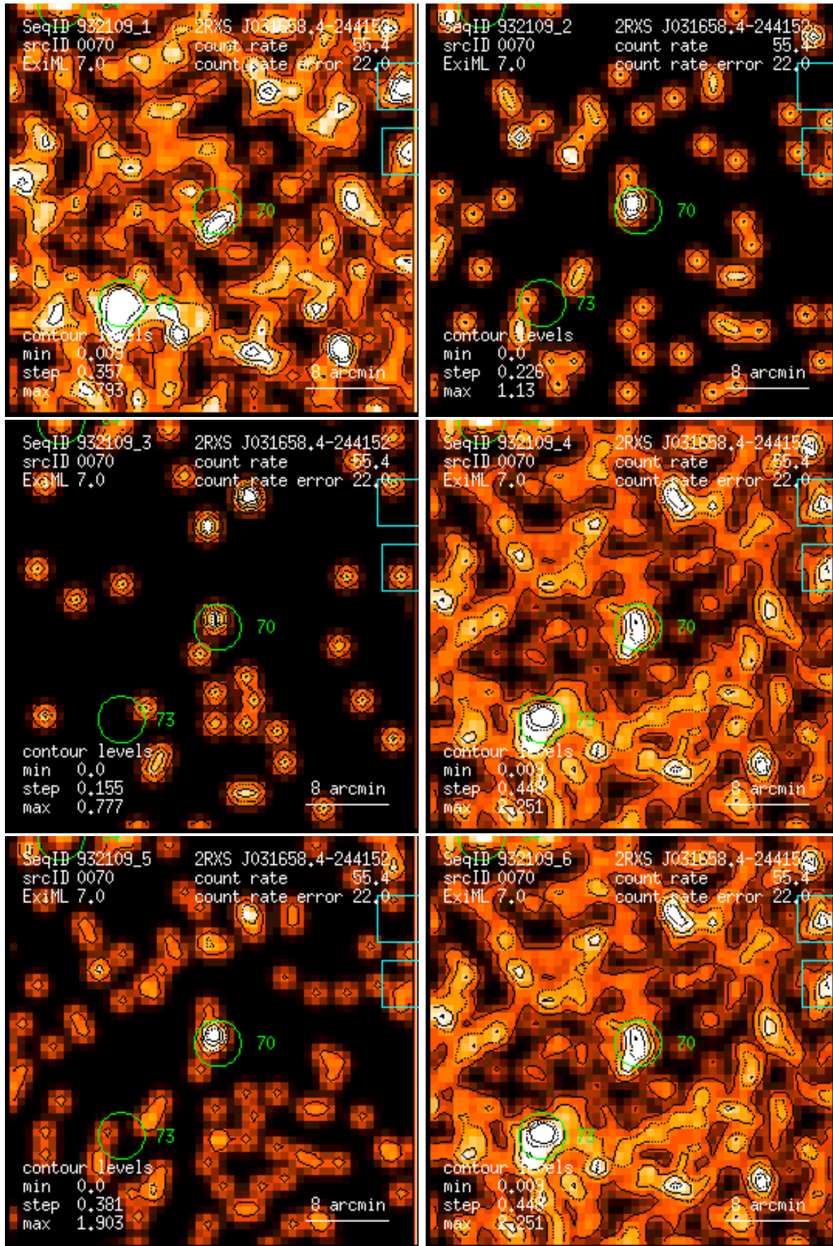
Figure 70: RASS 932109: detection 0070: band rate images, Gaussian filter: (1) PSPC channels 11 – 41, (2) 52 – 90, (3) 91 – 201, (4) 11 – 235, (5) 52 – 201, (6) 11 – 201. Broad band rates in counts/ks. Band rate contour levels in counts/ks/arcmin 2 .
