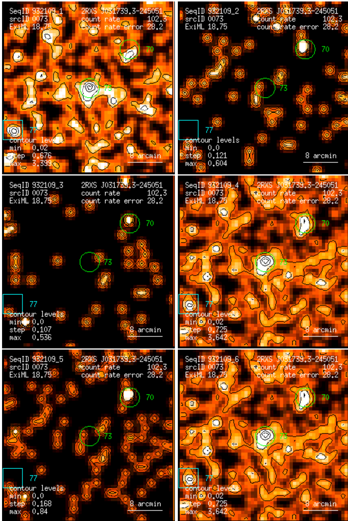
Figure 73: RASS 932109: detection 0073: band rate images, Gaussian filter: (1) PSPC channels 11 – 41, (2) 52 – 90, (3) 91 – 201, (4) 11 – 235, (5) 52 – 201, (6) 11 – 201. Broad band rates in counts/ks. Band rate contour levels in counts/ks/arcmin 2 .
