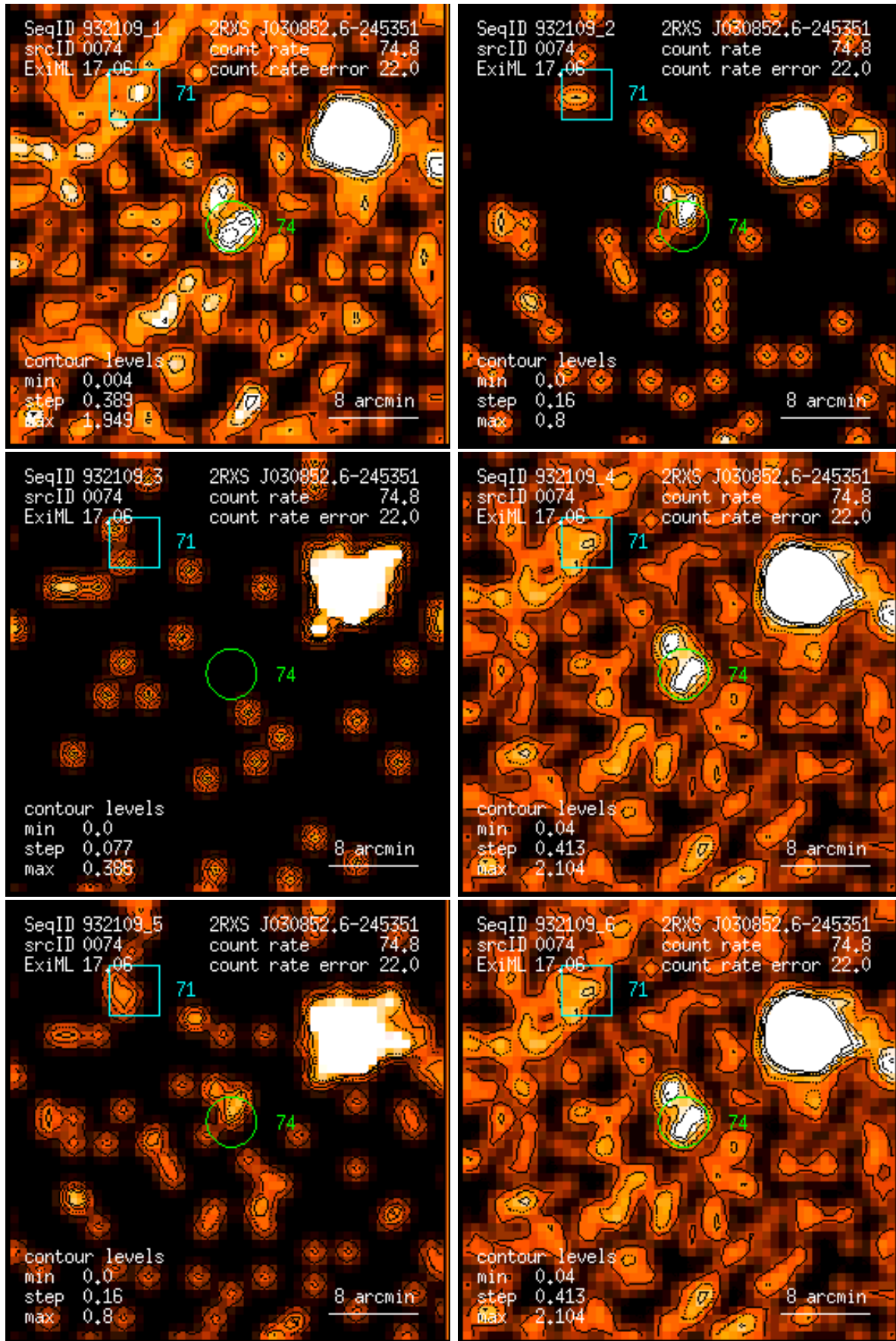
Figure 74: RASS 932109: detection 0074: band rate images, Gaussian filter: (1) PSPC channels 11 – 41, (2) 52 – 90, (3) 91 – 201, (4) 11 – 235, (5) 52 – 201, (6) 11 – 201. Broad band rates in counts/ks. Band rate contour levels in counts/ks/arcmin 2 .
