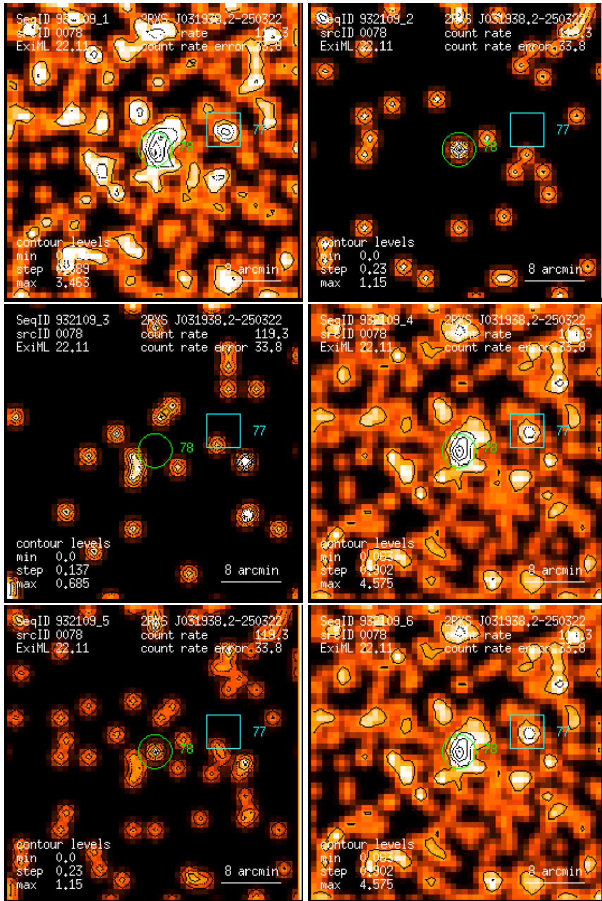
Figure 78: RASS 932109: detection 0078: band rate images, Gaussian filter: (1) PSPC channels 11 – 41, (2) 52 – 90, (3) 91 – 201, (4) 11 – 235, (5) 52 – 201, (6) 11 – 201. Broad band rates in counts/ks. Band rate contour levels in counts/ks/arcmin 2 .
