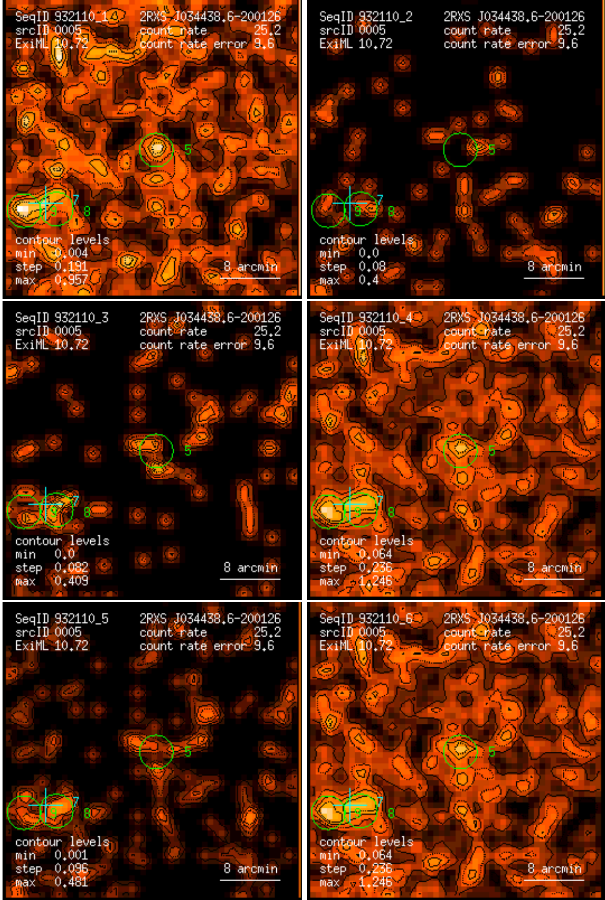
Figure 5: RASS 932110: detection 0005: band rate images, Gaussian filter: (1) PSPC channels 11 – 41, (2) 52 – 90, (3) 91 – 201, (4) 11 – 235, (5) 52 – 201, (6) 11 – 201. Broad band rates in counts/ks. Band rate contour levels in counts/ks/arcmin 2 .
