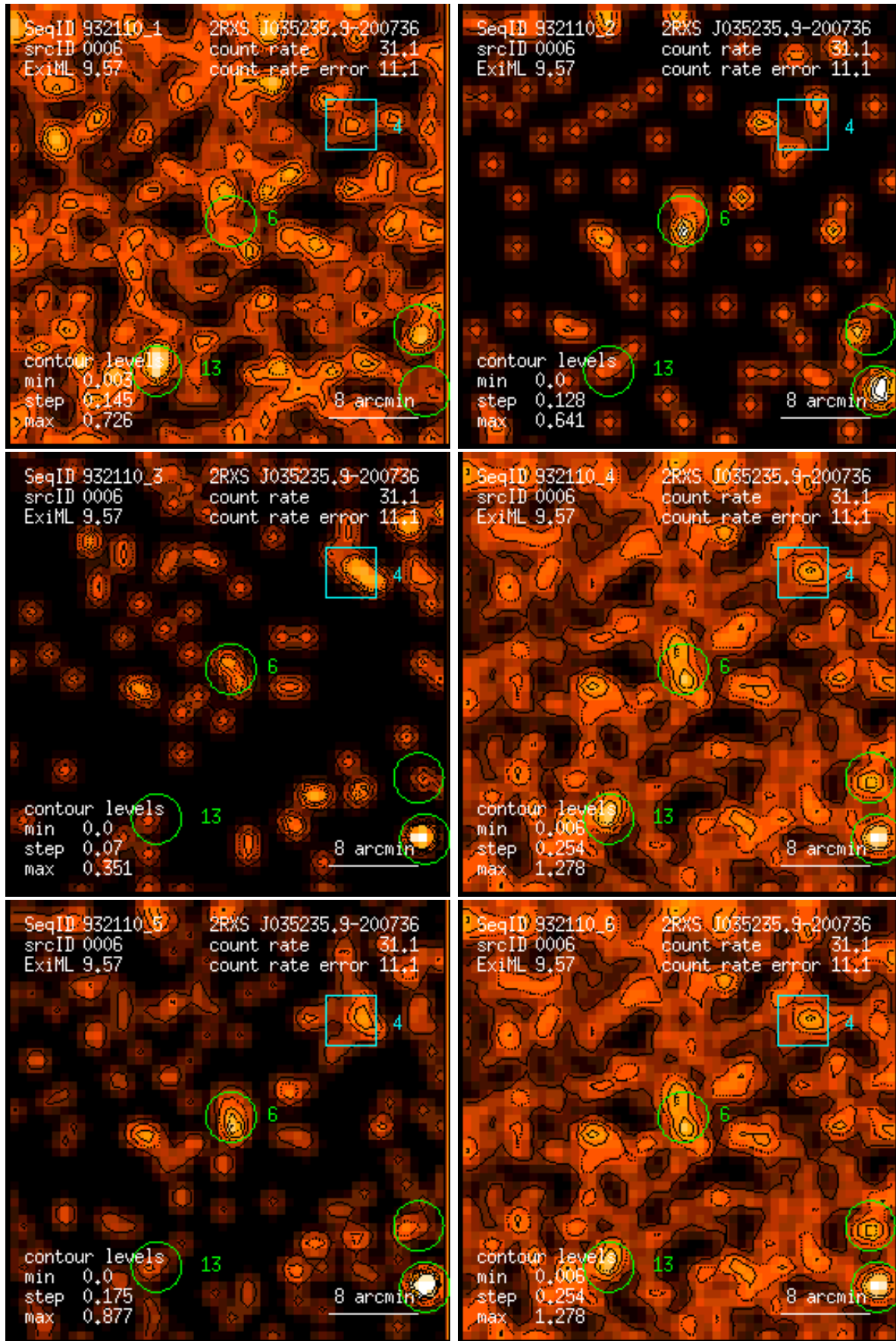
Figure 6: RASS 932110: detection 0006: band rate images, Gaussian filter: (1) PSPC channels 11 – 41, (2) 52 – 90, (3) 91 – 201, (4) 11 – 235, (5) 52 – 201, (6) 11 – 201. Broad band rates in counts/ks. Band rate contour levels in counts/ks/arcmin 2 .
