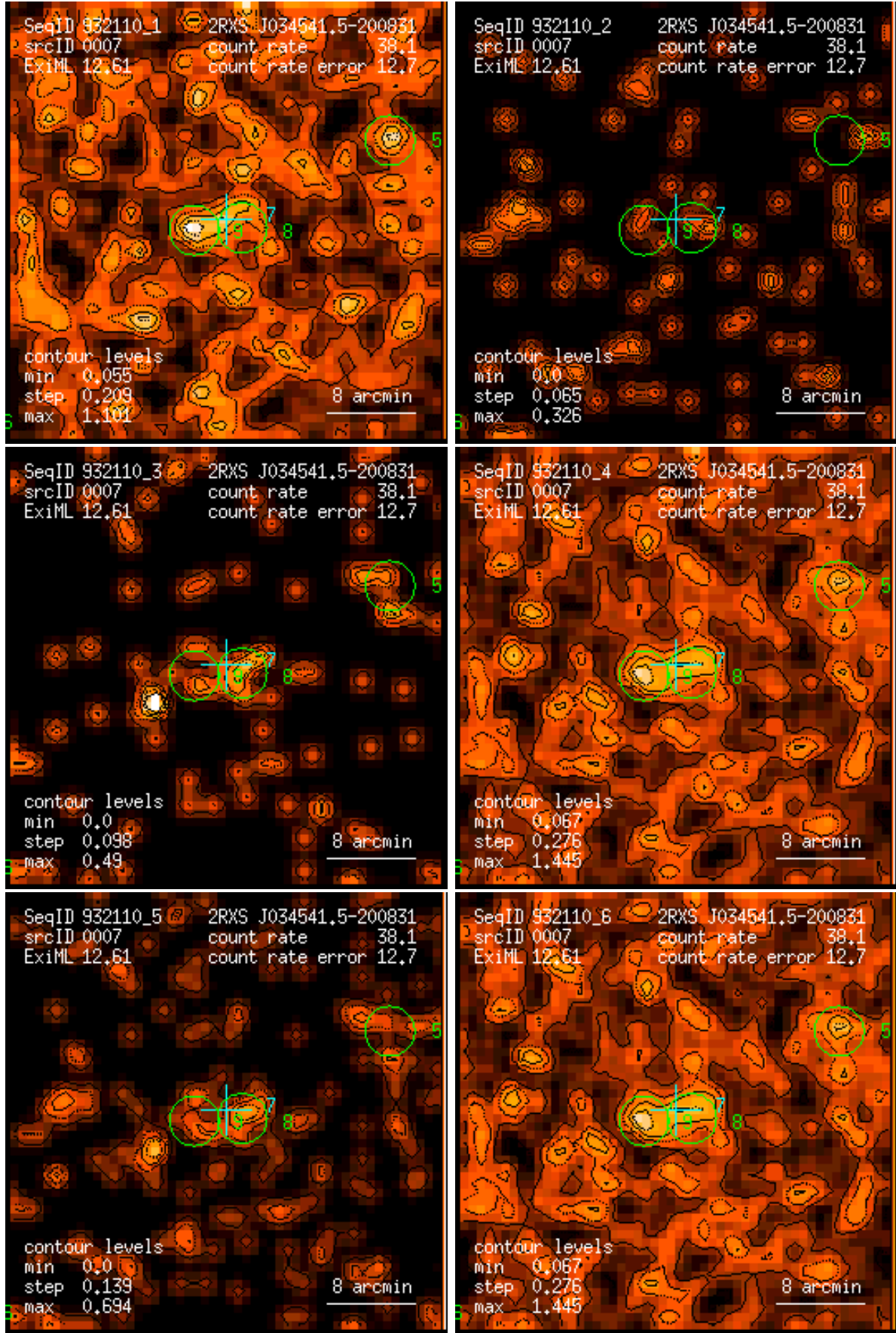
Figure 7: RASS 932110: detection 0007: band rate images, Gaussian filter: (1) PSPC channels 11 – 41, (2) 52 – 90, (3) 91 – 201, (4) 11 – 235, (5) 52 – 201, (6) 11 – 201. Broad band rates in counts/ks. Band rate contour levels in counts/ks/arcmin 2 .
