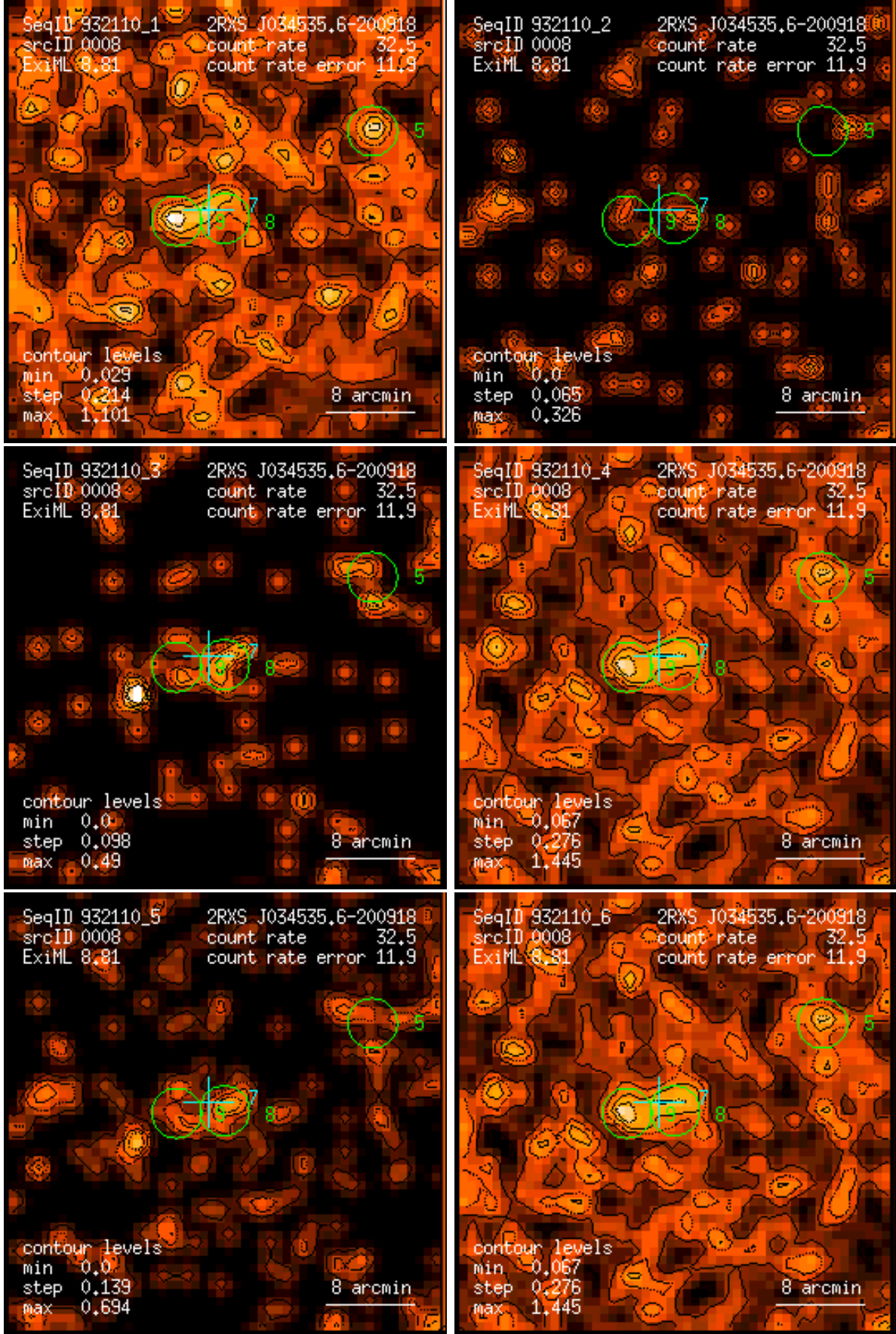
Figure 8: RASS 932110: detection 0008: band rate images, Gaussian filter: (1) PSPC channels 11 – 41, (2) 52 – 90, (3) 91 – 201, (4) 11 – 235, (5) 52 – 201, (6) 11 – 201. Broad band rates in counts/ks. Band rate contour levels in counts/ks/arcmin 2 .
