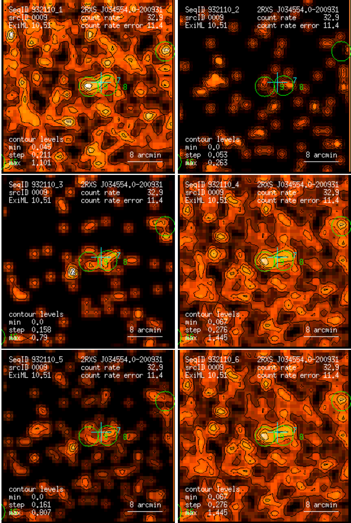
Figure 9: RASS 932110: detection 0009: band rate images, Gaussian filter: (1) PSPC channels 11 – 41, (2) 52 – 90, (3) 91 – 201, (4) 11 – 235, (5) 52 – 201, (6) 11 – 201. Broad band rates in counts/ks. Band rate contour levels in counts/ks/arcmin 2 .
