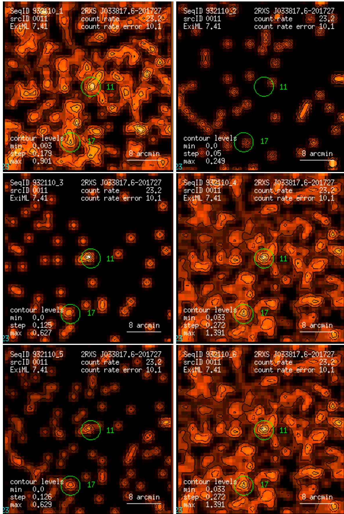
Figure 11: RASS 932110: detection 0011: band rate images, Gaussian filter: (1) PSPC channels 11 – 41, (2) 52 – 90, (3) 91 – 201, (4) 11 – 235, (5) 52 – 201, (6) 11 – 201. Broad band rates in counts/ks. Band rate contour levels in counts/ks/arcmin 2 .
