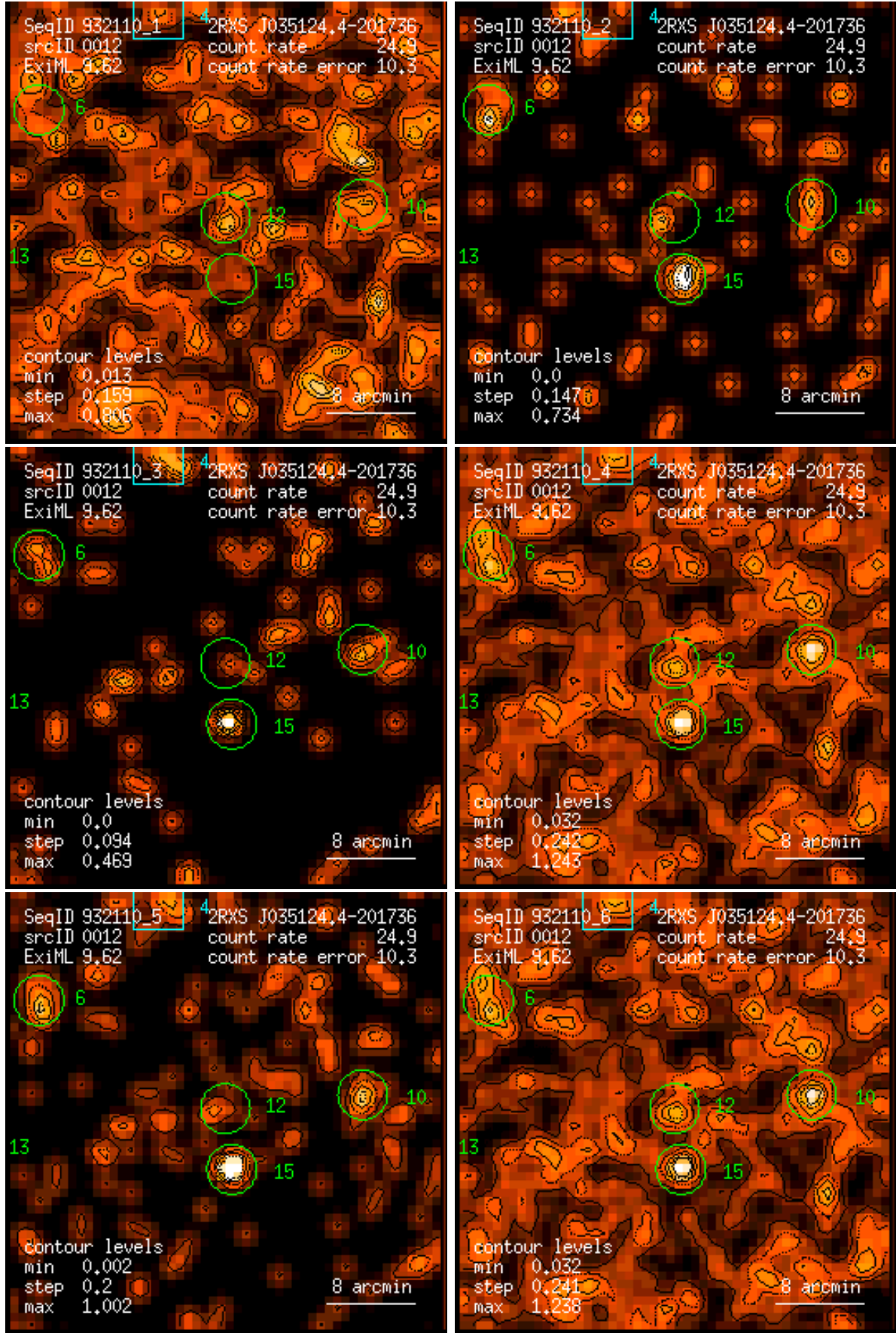
Figure 12: RASS 932110: detection 0012: band rate images, Gaussian filter: (1) PSPC channels 11 – 41, (2) 52 – 90, (3) 91 – 201, (4) 11 – 235, (5) 52 – 201, (6) 11 – 201. Broad band rates in counts/ks. Band rate contour levels in counts/ks/arcmin 2 .
