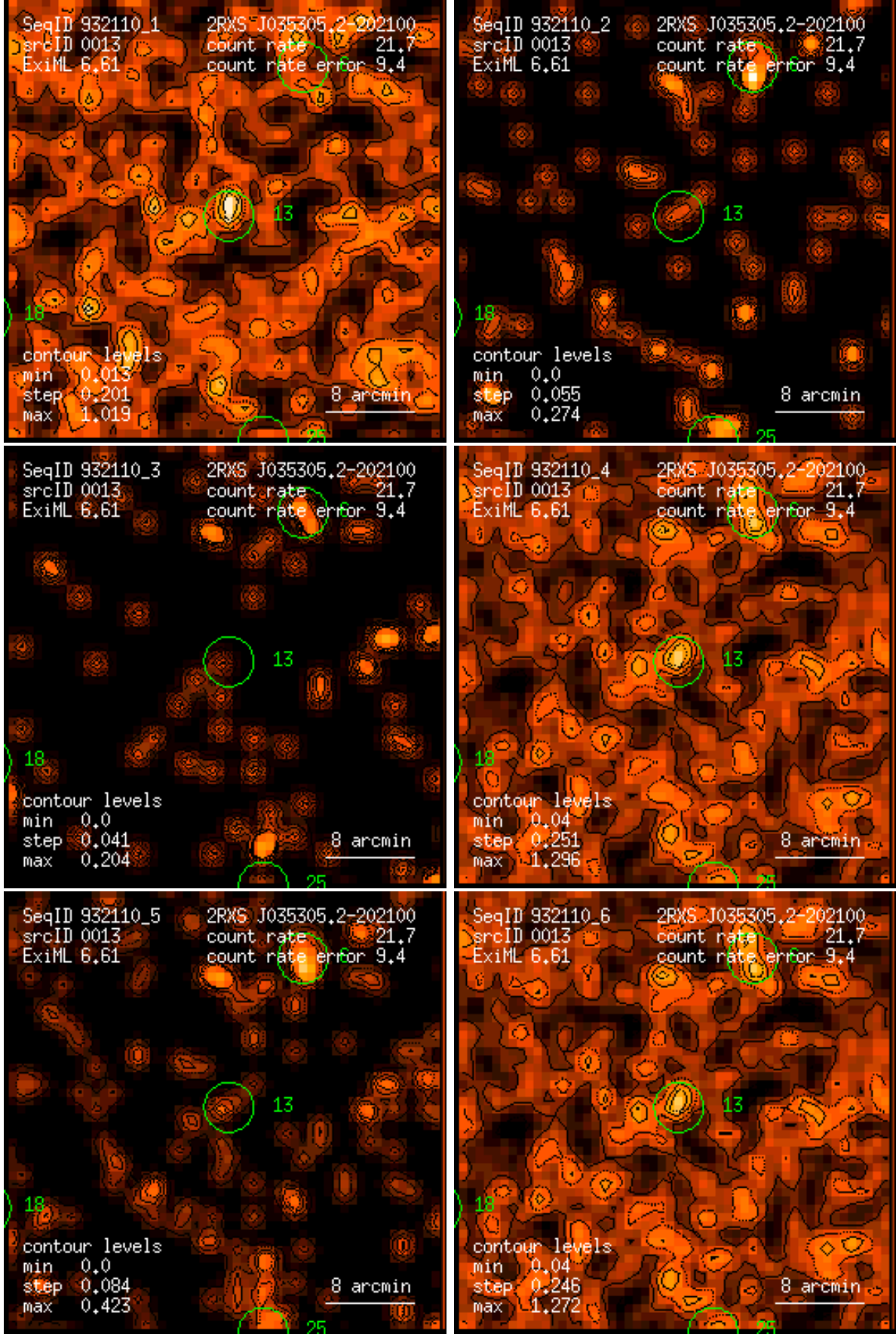
Figure 13: RASS 932110: detection 0013: band rate images, Gaussian filter: (1) PSPC channels 11 – 41, (2) 52 – 90, (3) 91 – 201, (4) 11 – 235, (5) 52 – 201, (6) 11 – 201. Broad band rates in counts/ks. Band rate contour levels in counts/ks/arcmin 2 .
