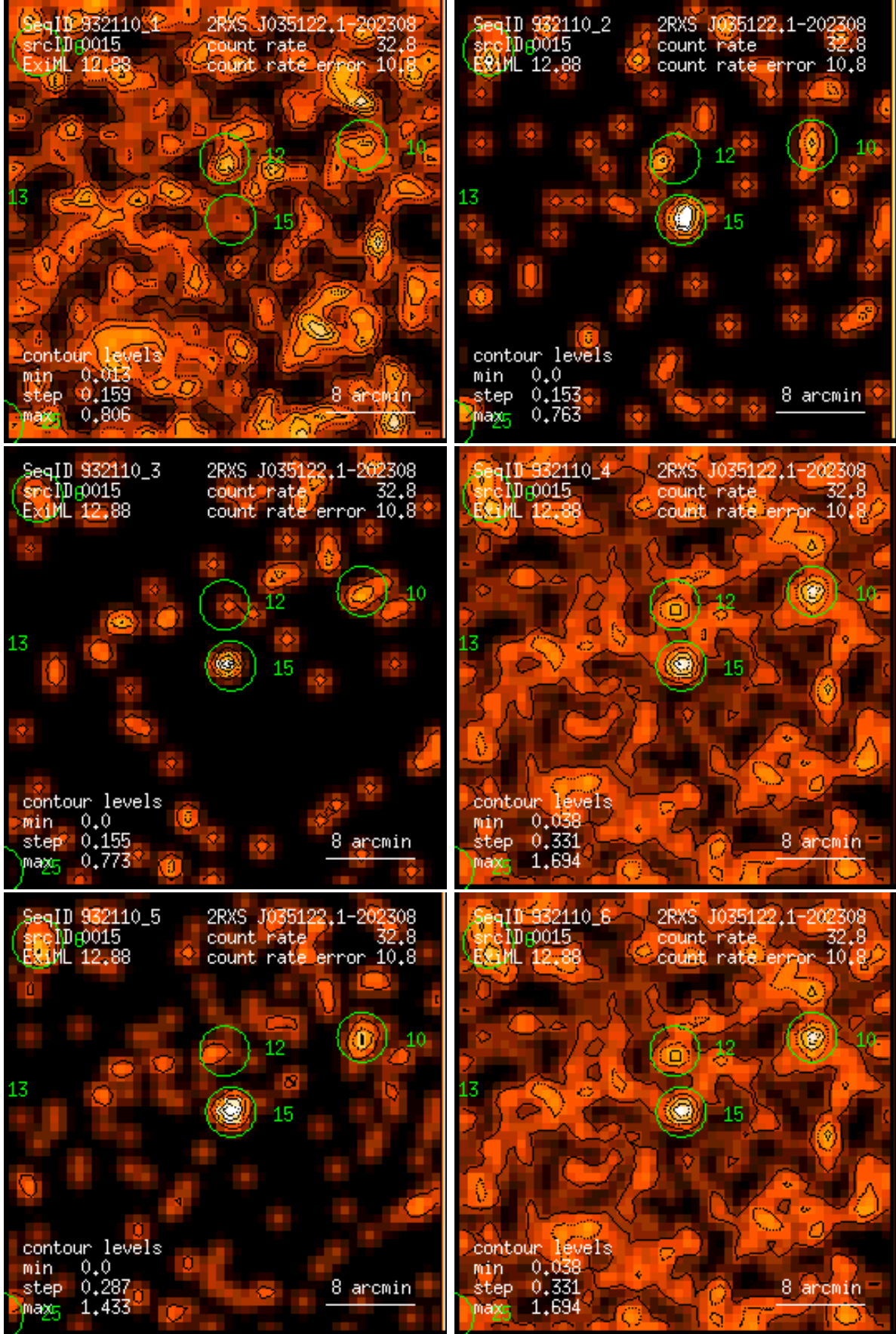
Figure 15: RASS 932110: detection 0015: band rate images, Gaussian filter: (1) PSPC channels 11 – 41, (2) 52 – 90, (3) 91 – 201, (4) 11 – 235, (5) 52 – 201, (6) 11 – 201. Broad band rates in counts/ks. Band rate contour levels in counts/ks/arcmin 2 .
