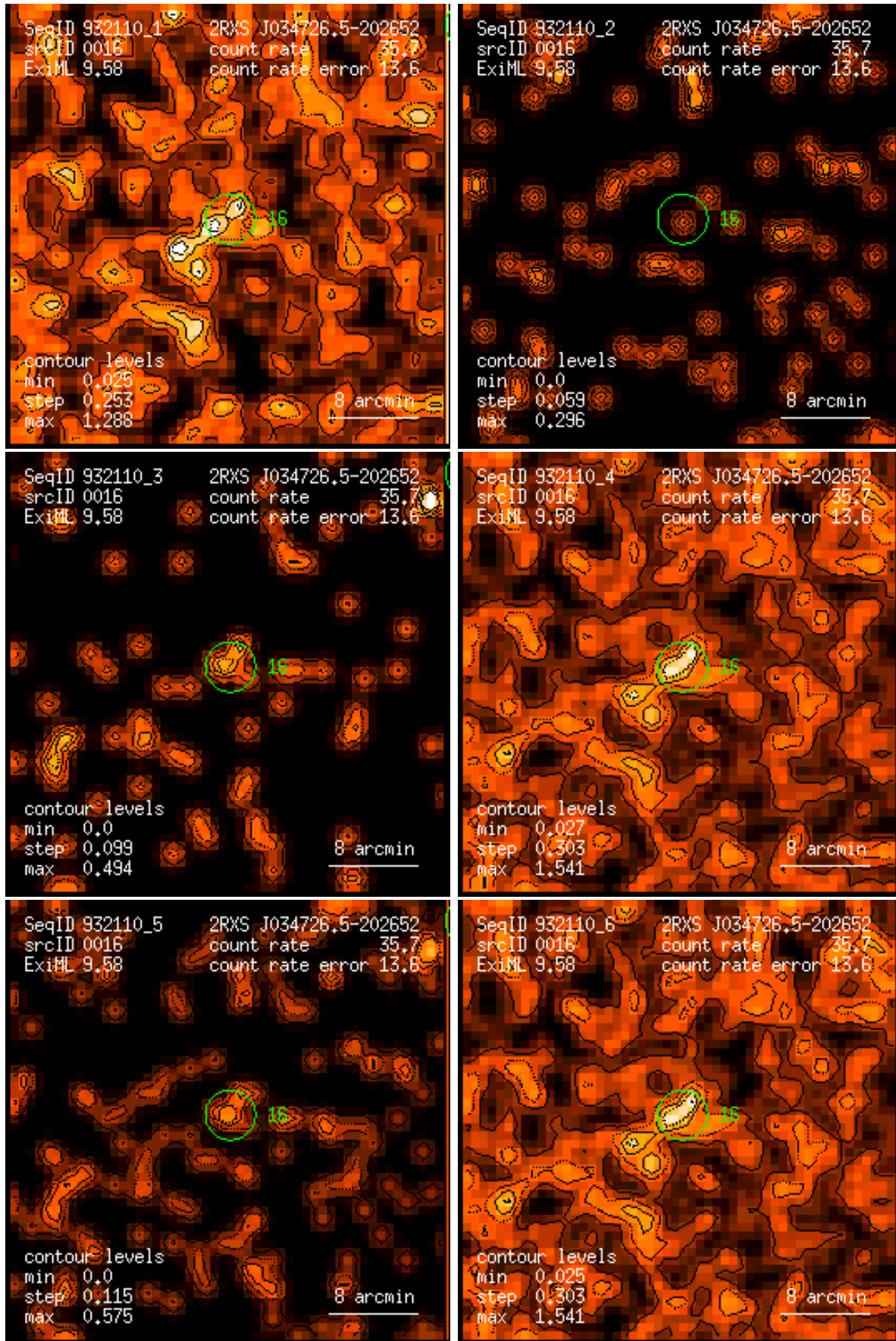
Figure 16: RASS 932110: detection 0016: band rate images, Gaussian filter: (1) PSPC channels 11 – 41, (2) 52 – 90, (3) 91 – 201, (4) 11 – 235, (5) 52 – 201, (6) 11 – 201. Broad band rates in counts/ks. Band rate contour levels in counts/ks/arcmin 2 .
