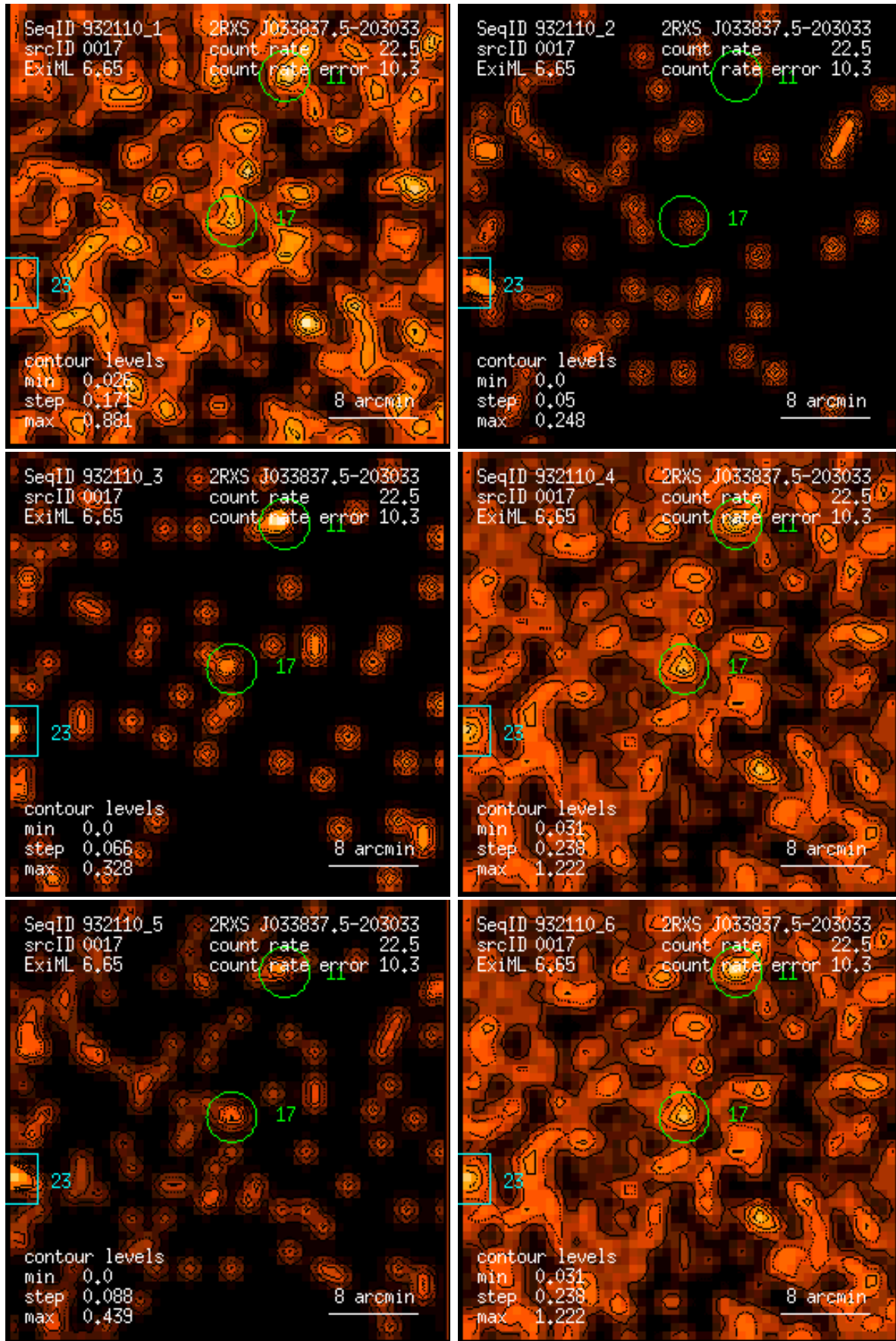
Figure 17: RASS 932110: detection 0017: band rate images, Gaussian filter: (1) PSPC channels 11 – 41, (2) 52 – 90, (3) 91 – 201, (4) 11 – 235, (5) 52 – 201, (6) 11 – 201. Broad band rates in counts/ks. Band rate contour levels in counts/ks/arcmin 2 .
