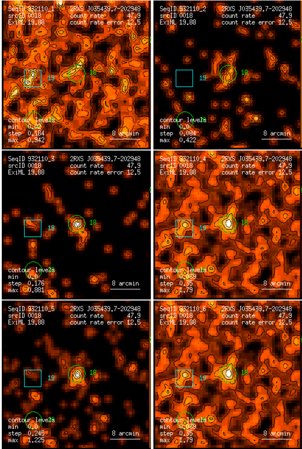
Figure 18: RASS 932110: detection 0018: band rate images, Gaussian filter: (1) PSPC channels 11 – 41, (2) 52 – 90, (3) 91 – 201, (4) 11 – 235, (5) 52 – 201, (6) 11 – 201. Broad band rates in counts/ks. Band rate contour levels in counts/ks/arcmin 2 .
