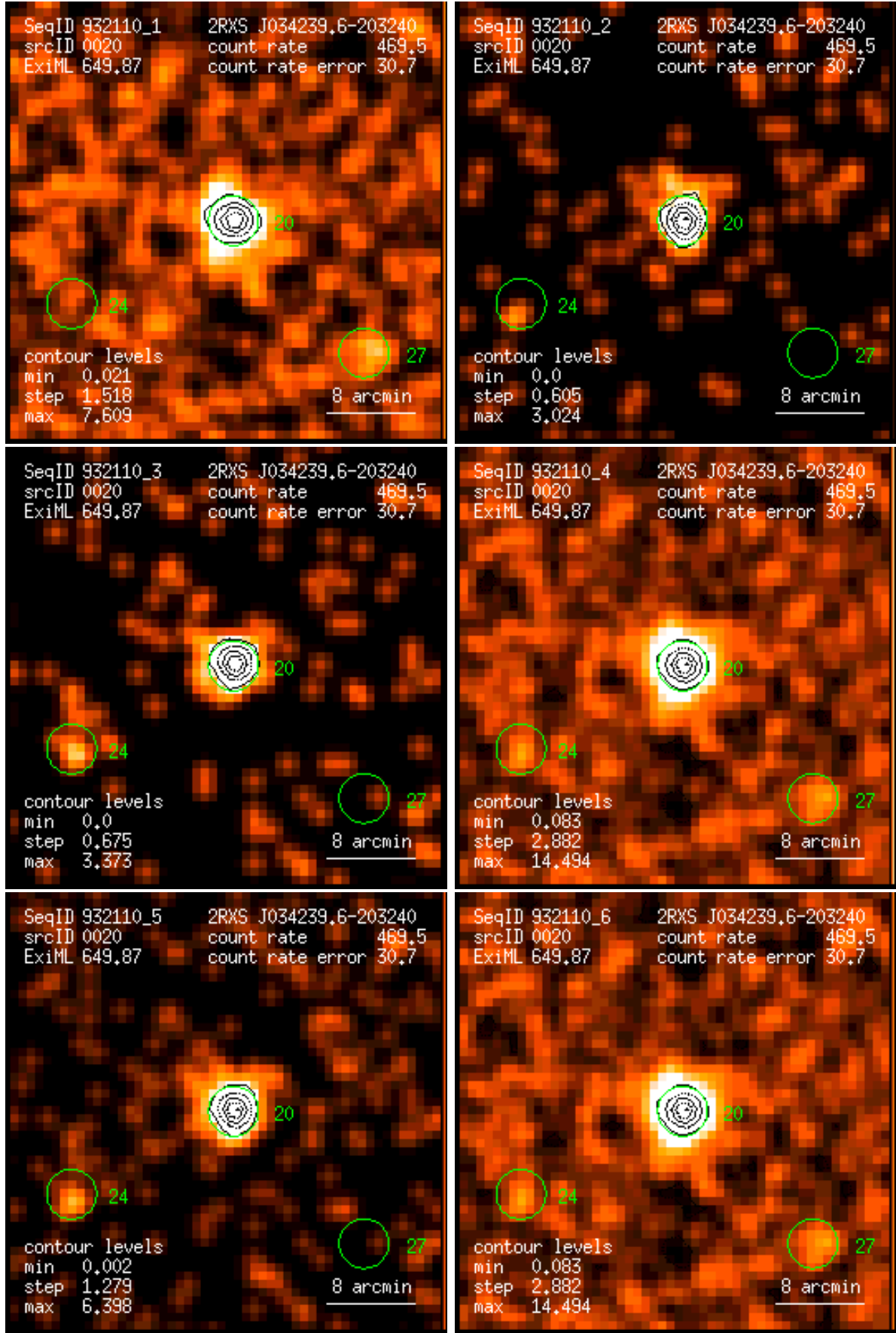
Figure 20: RASS 932110: detection 0020: band rate images, Gaussian filter: (1) PSPC channels 11 – 41, (2) 52 – 90, (3) 91 – 201, (4) 11 – 235, (5) 52 – 201, (6) 11 – 201. Broad band rates in counts/ks. Band rate contour levels in counts/ks/arcmin 2 .
