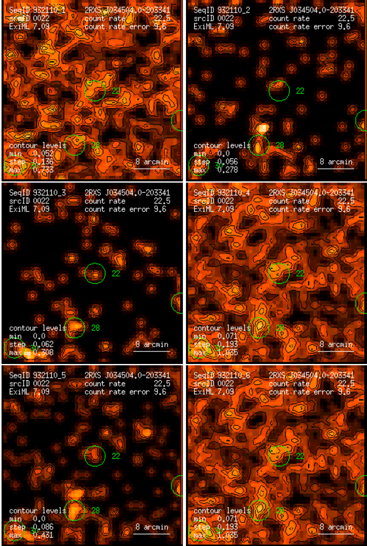
Figure 22: RASS 932110: detection 0022: band rate images, Gaussian filter: (1) PSPC channels 11 – 41, (2) 52 – 90, (3) 91 – 201, (4) 11 – 235, (5) 52 – 201, (6) 11 – 201. Broad band rates in counts/ks. Band rate contour levels in counts/ks/arcmin 2 .
