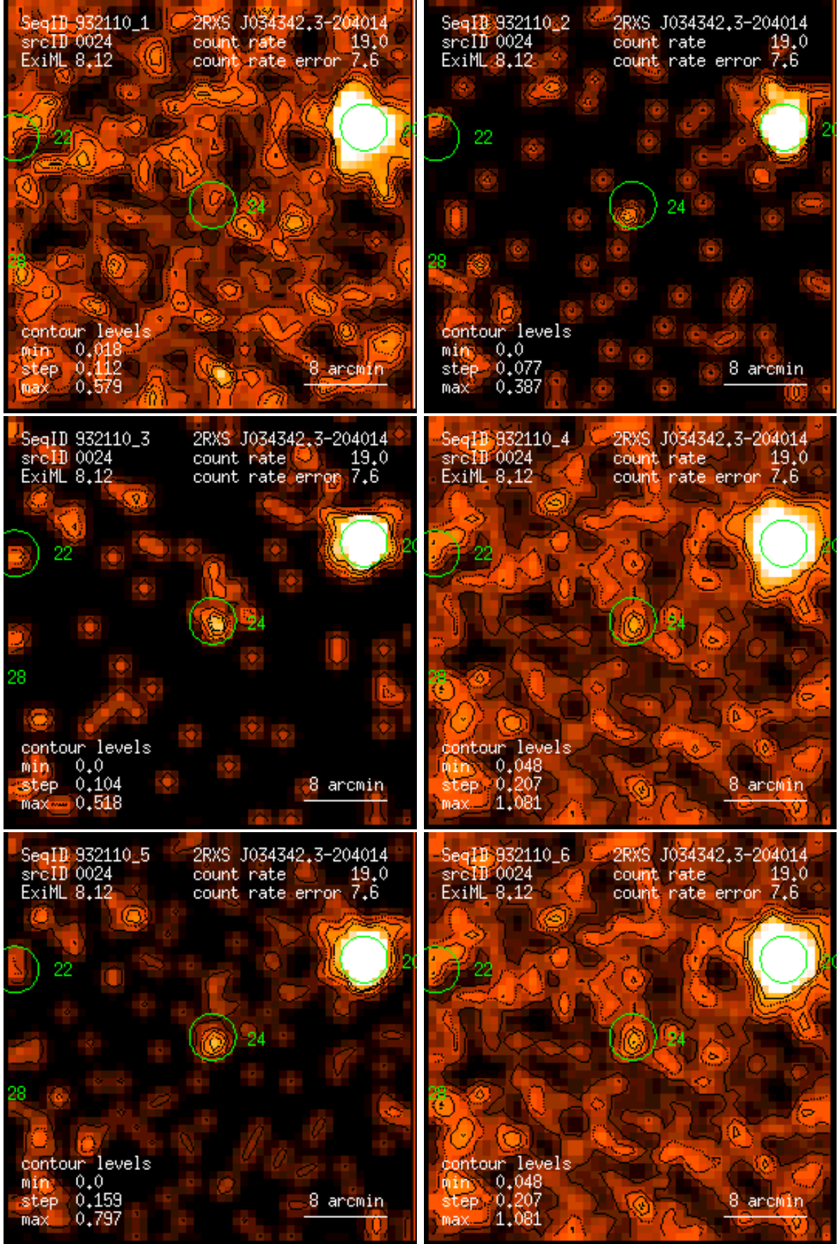
Figure 24: RASS 932110: detection 0024: band rate images, Gaussian filter: (1) PSPC channels 11 – 41, (2) 52 – 90, (3) 91 – 201, (4) 11 – 235, (5) 52 – 201, (6) 11 – 201. Broad band rates in counts/ks. Band rate contour levels in counts/ks/arcmin 2 .
