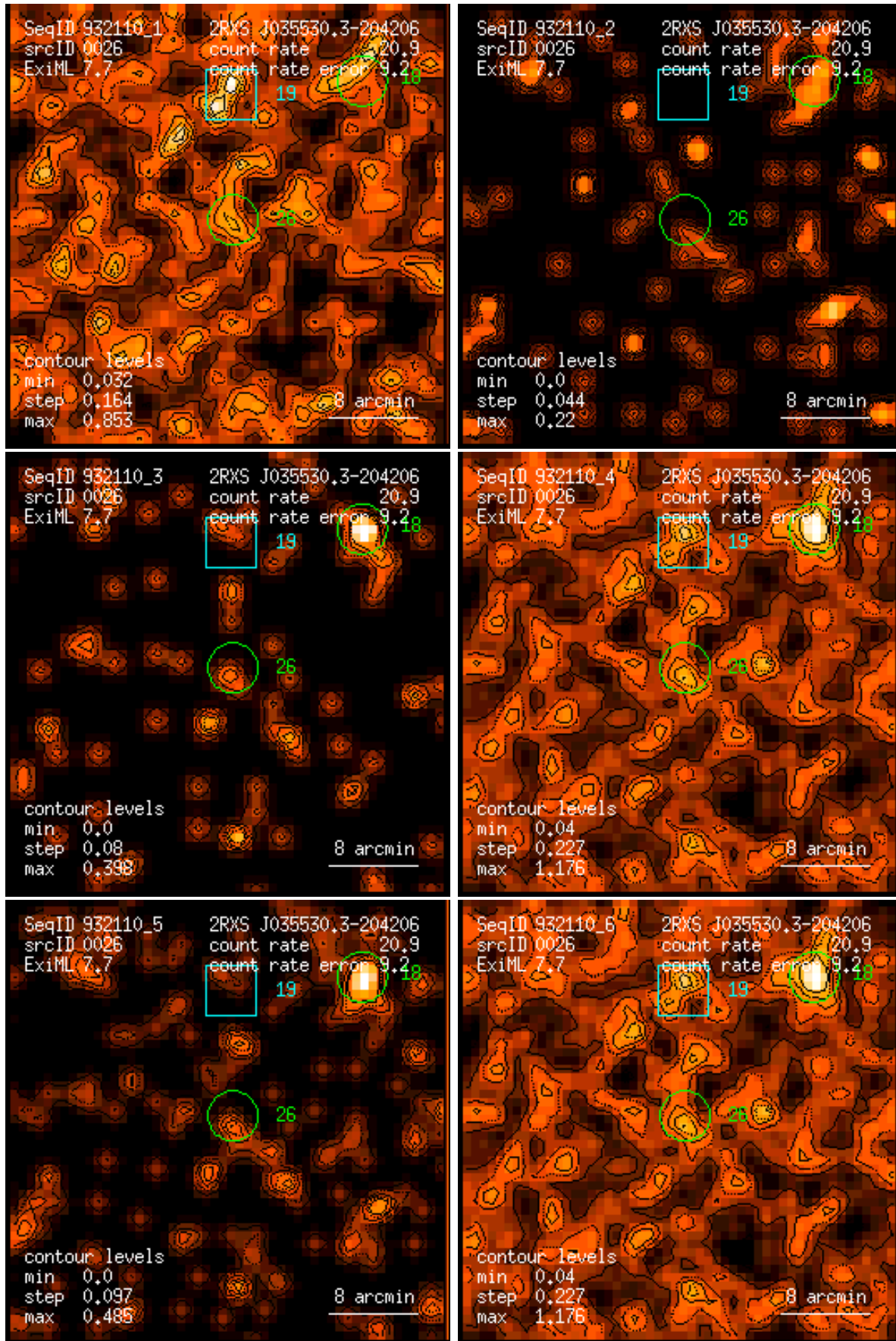
Figure 26: RASS 932110: detection 0026: band rate images, Gaussian filter: (1) PSPC channels 11 – 41, (2) 52 – 90, (3) 91 – 201, (4) 11 – 235, (5) 52 – 201, (6) 11 – 201. Broad band rates in counts/ks. Band rate contour levels in counts/ks/arcmin 2 .
