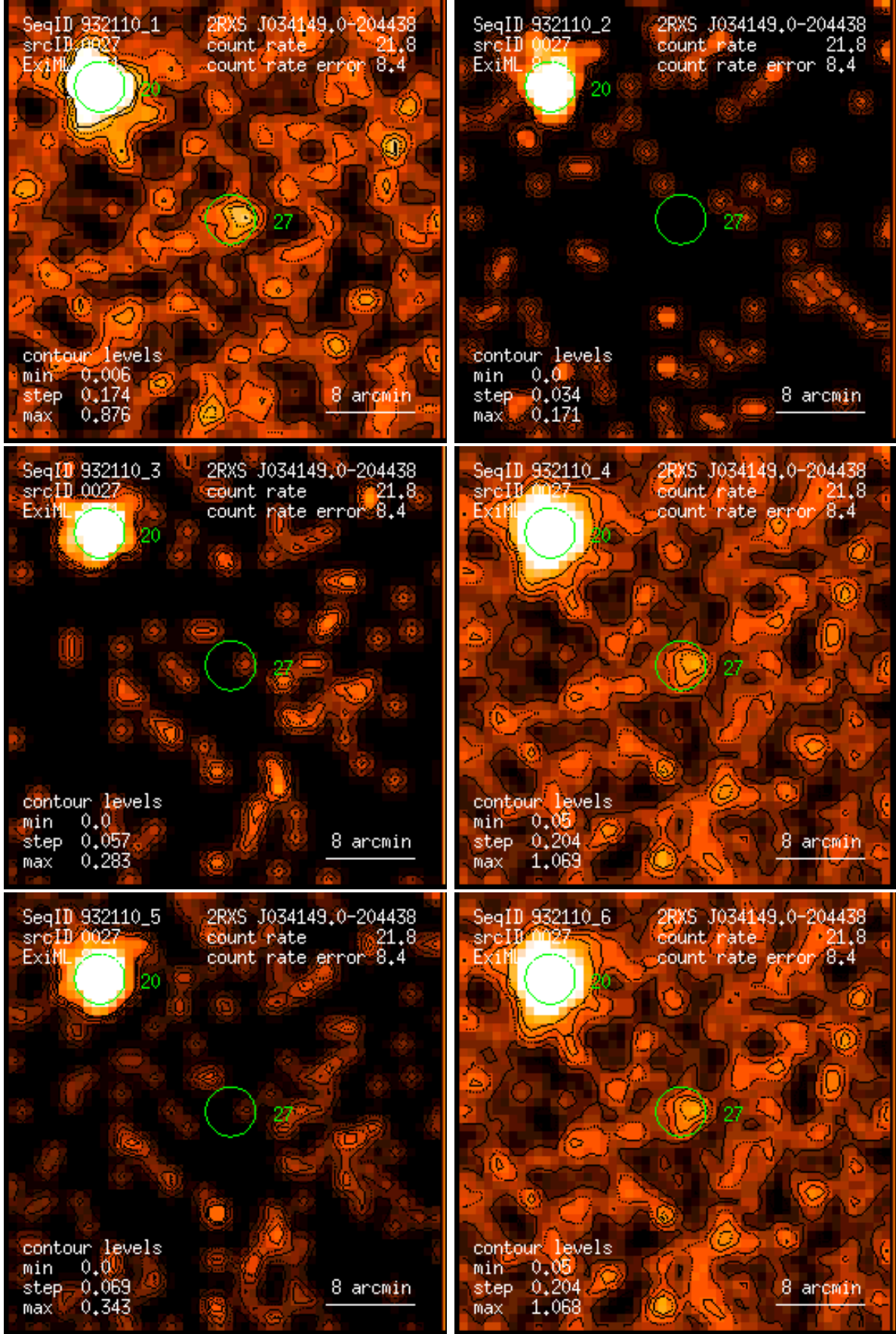
Figure 27: RASS 932110: detection 0027: band rate images, Gaussian filter: (1) PSPC channels 11 – 41, (2) 52 – 90, (3) 91 – 201, (4) 11 – 235, (5) 52 – 201, (6) 11 – 201. Broad band rates in counts/ks. Band rate contour levels in counts/ks/arcmin 2 .
