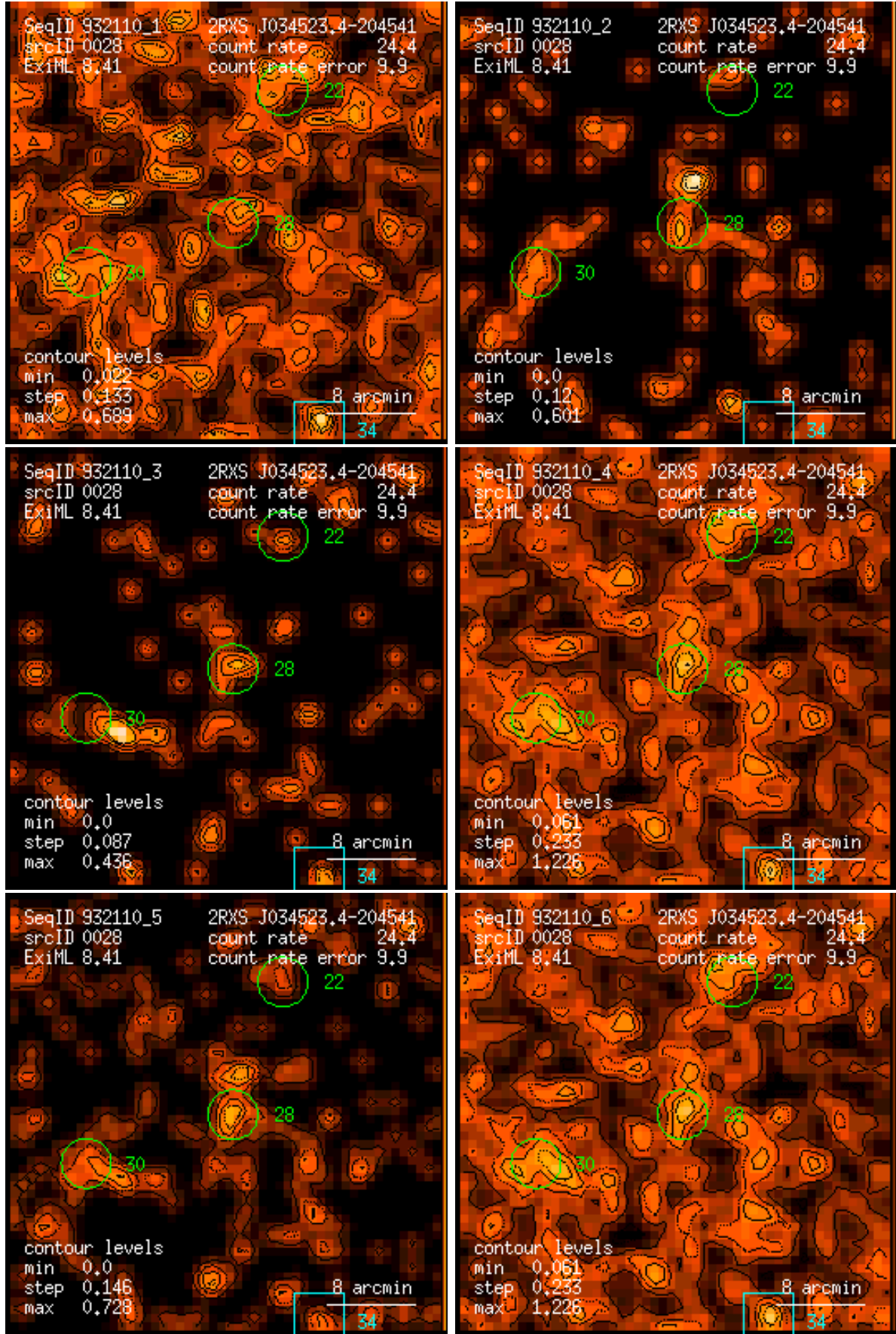
Figure 28: RASS 932110: detection 0028: band rate images, Gaussian filter: (1) PSPC channels 11 – 41, (2) 52 – 90, (3) 91 – 201, (4) 11 – 235, (5) 52 – 201, (6) 11 – 201. Broad band rates in counts/ks. Band rate contour levels in counts/ks/arcmin 2 .
