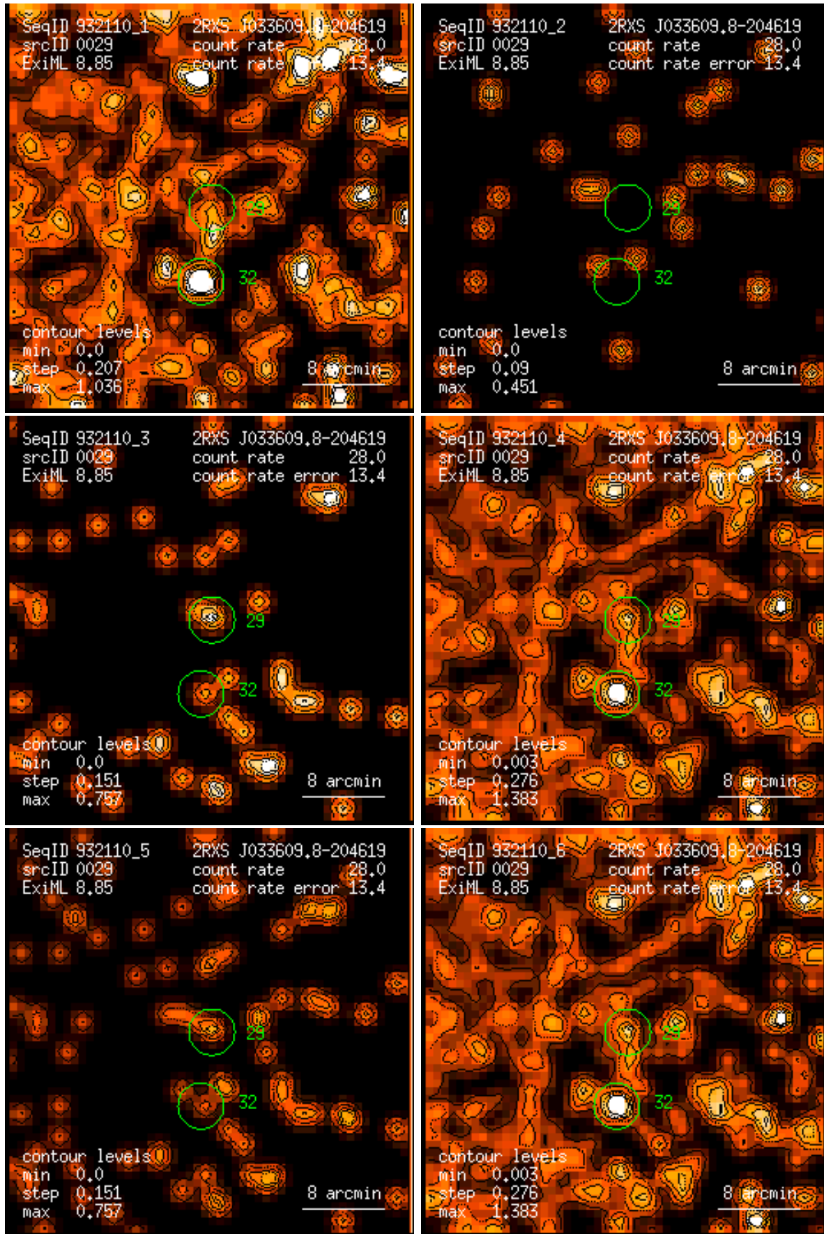
Figure 29: RASS 932110: detection 0029: band rate images, Gaussian filter: (1) PSPC channels 11 – 41, (2) 52 – 90, (3) 91 – 201, (4) 11 – 235, (5) 52 – 201, (6) 11 – 201. Broad band rates in counts/ks. Band rate contour levels in counts/ks/arcmin 2 .
