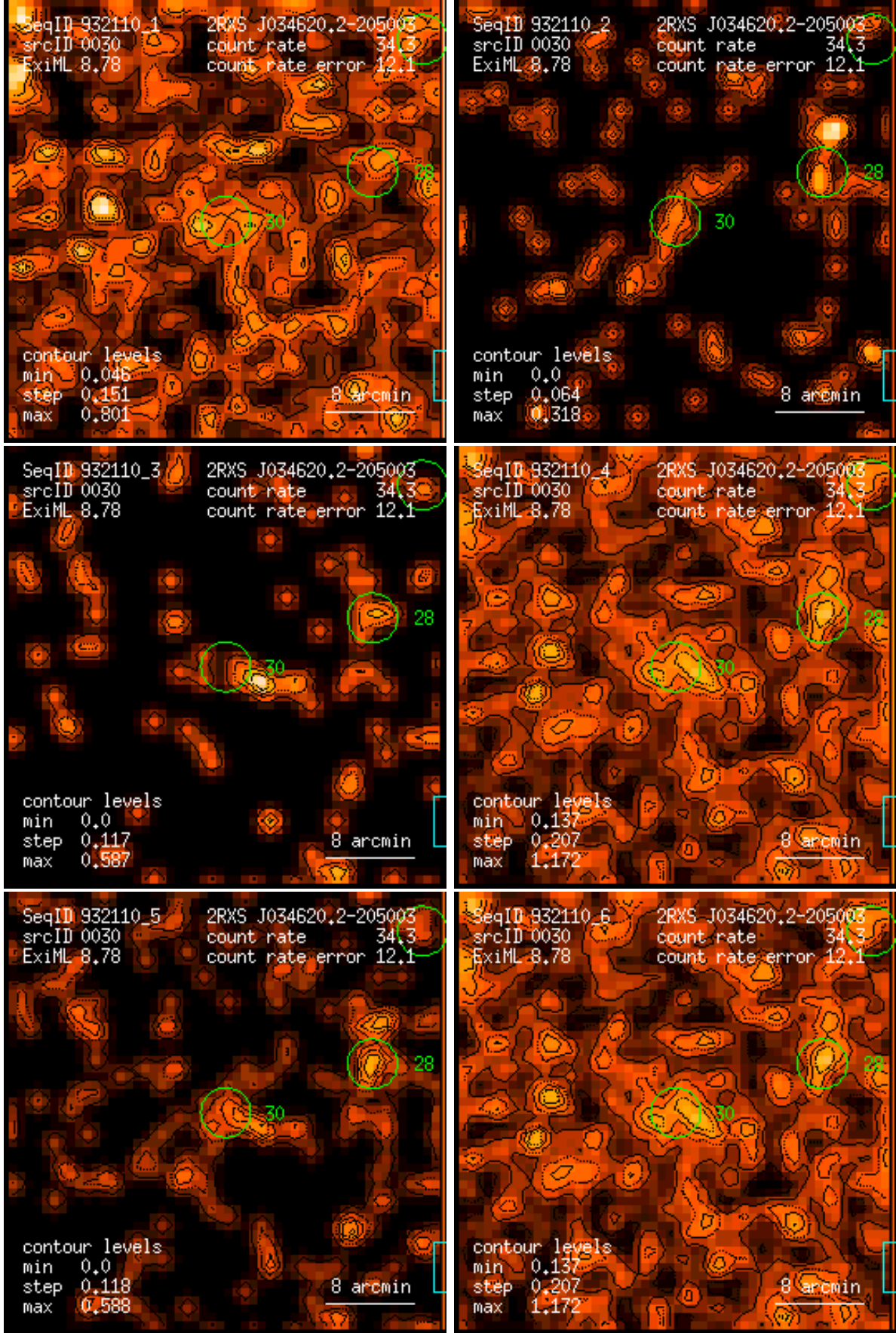
Figure 30: RASS 932110: detection 0030: band rate images, Gaussian filter: (1) PSPC channels 11 – 41, (2) 52 – 90, (3) 91 – 201, (4) 11 – 235, (5) 52 – 201, (6) 11 – 201. Broad band rates in counts/ks. Band rate contour levels in counts/ks/arcmin 2 .
