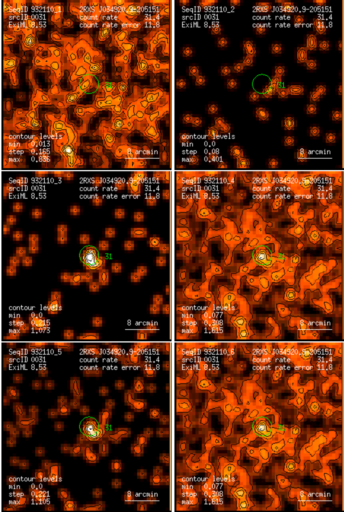
Figure 31: RASS 932110: detection 0031: band rate images, Gaussian filter: (1) PSPC channels 11 – 41, (2) 52 – 90, (3) 91 – 201, (4) 11 – 235, (5) 52 – 201, (6) 11 – 201. Broad band rates in counts/ks. Band rate contour levels in counts/ks/arcmin 2 .
