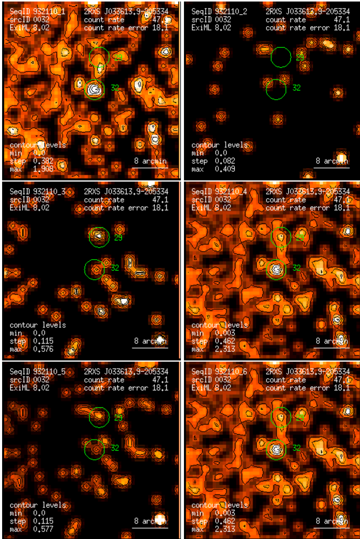
Figure 32: RASS 932110: detection 0032: band rate images, Gaussian filter: (1) PSPC channels 11 – 41, (2) 52 – 90, (3) 91 – 201, (4) 11 – 235, (5) 52 – 201, (6) 11 – 201. Broad band rates in counts/ks. Band rate contour levels in counts/ks/arcmin 2 .
