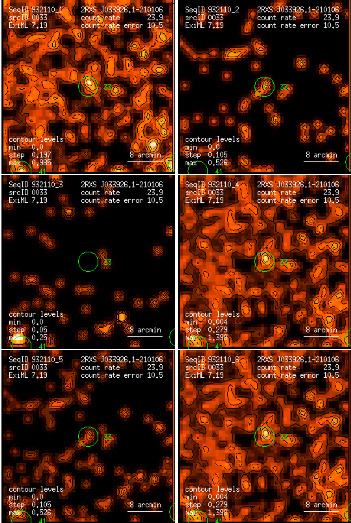
Figure 33: RASS 932110: detection 0033: band rate images, Gaussian filter: (1) PSPC channels 11 – 41, (2) 52 – 90, (3) 91 – 201, (4) 11 – 235, (5) 52 – 201, (6) 11 – 201. Broad band rates in counts/ks. Band rate contour levels in counts/ks/arcmin 2 .
