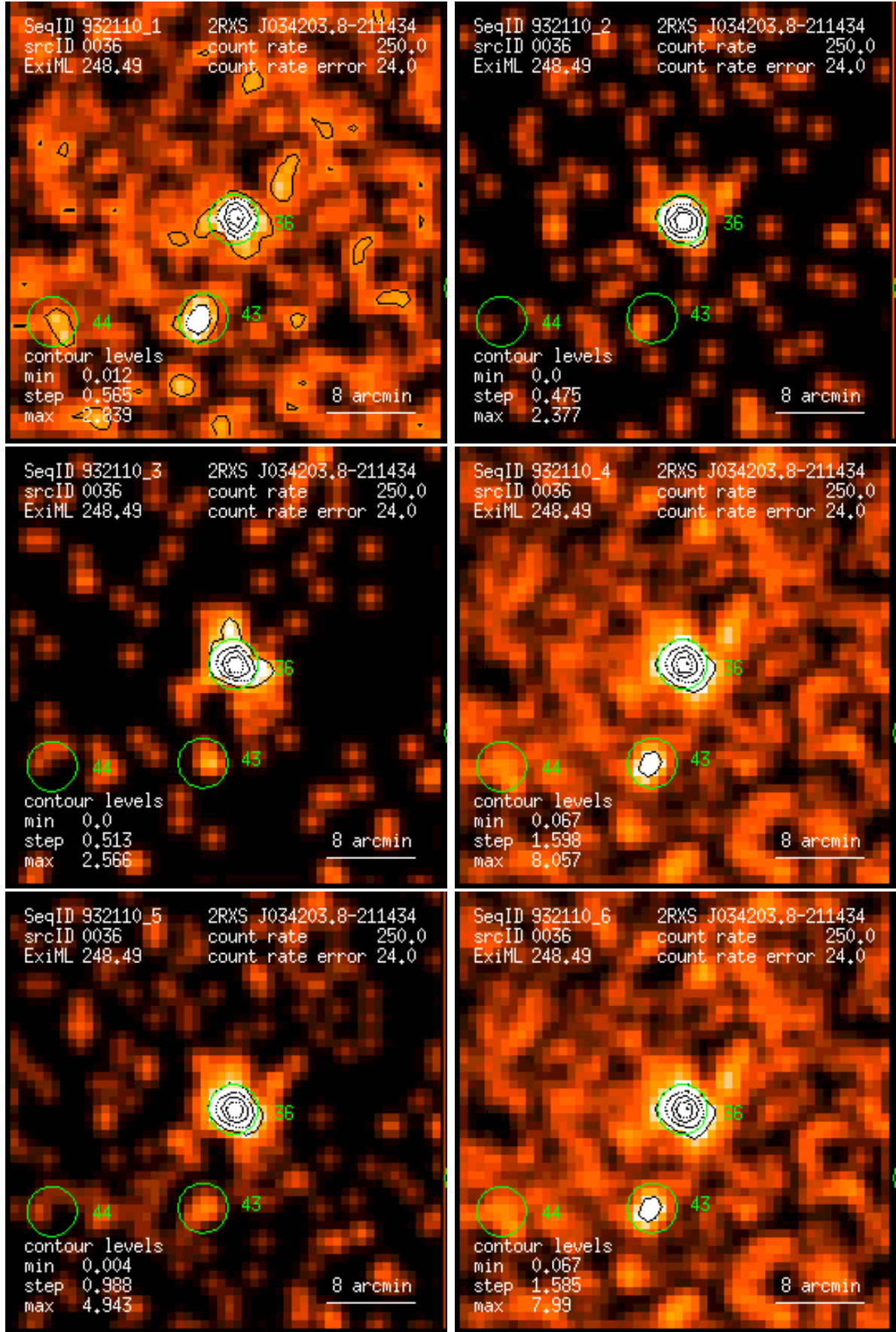
Figure 36: RASS 932110: detection 0036: band rate images, Gaussian filter: (1) PSPC channels 11 – 41, (2) 52 – 90, (3) 91 – 201, (4) 11 – 235, (5) 52 – 201, (6) 11 – 201. Broad band rates in counts/ks. Band rate contour levels in counts/ks/arcmin 2 .
