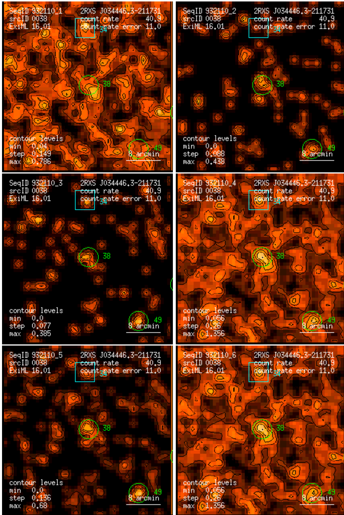
Figure 38: RASS 932110: detection 0038: band rate images, Gaussian filter: (1) PSPC channels 11 – 41, (2) 52 – 90, (3) 91 – 201, (4) 11 – 235, (5) 52 – 201, (6) 11 – 201. Broad band rates in counts/ks. Band rate contour levels in counts/ks/arcmin 2 .
