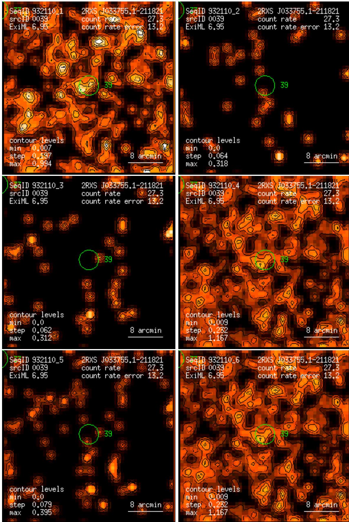
Figure 39: RASS 932110: detection 0039: band rate images, Gaussian filter: (1) PSPC channels 11 – 41, (2) 52 – 90, (3) 91 – 201, (4) 11 – 235, (5) 52 – 201, (6) 11 – 201. Broad band rates in counts/ks. Band rate contour levels in counts/ks/arcmin 2 .
