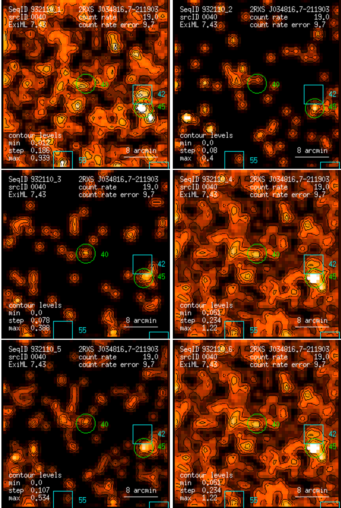
Figure 40: RASS 932110: detection 0040: band rate images, Gaussian filter: (1) PSPC channels 11 – 41, (2) 52 – 90, (3) 91 – 201, (4) 11 – 235, (5) 52 – 201, (6) 11 – 201. Broad band rates in counts/ks. Band rate contour levels in counts/ks/arcmin 2 .
